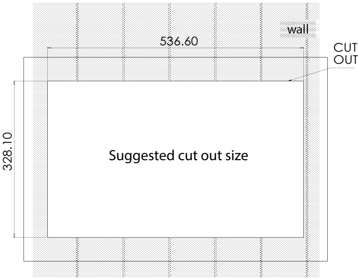
21.5" Panel mount cut out
