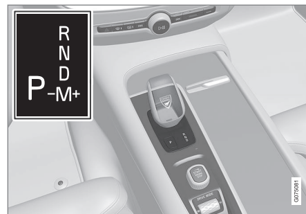
Overview of small gear selector and gear shift pattern in the instrument panel.
