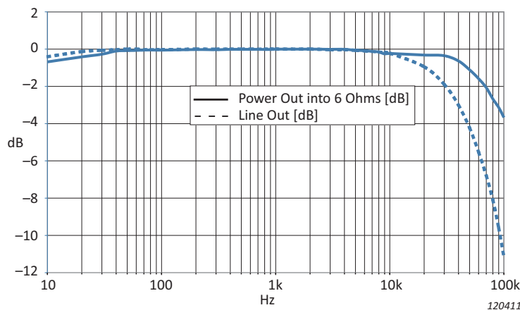
Fig. 1 Frequency Responses measured at a 0 dB output power of 300 W into 6 Ω up to 20 kHz and of 20 W up from 20 kHz
