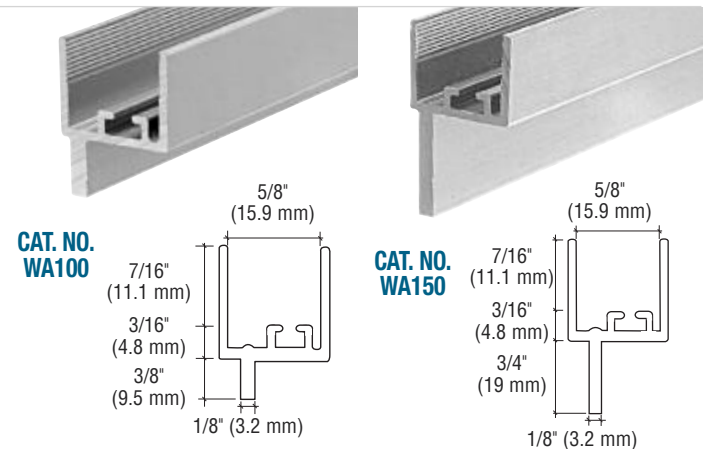
Offset Set Insulating Glass Adapter Channel for Sliding Bypassing Windows and Doors
