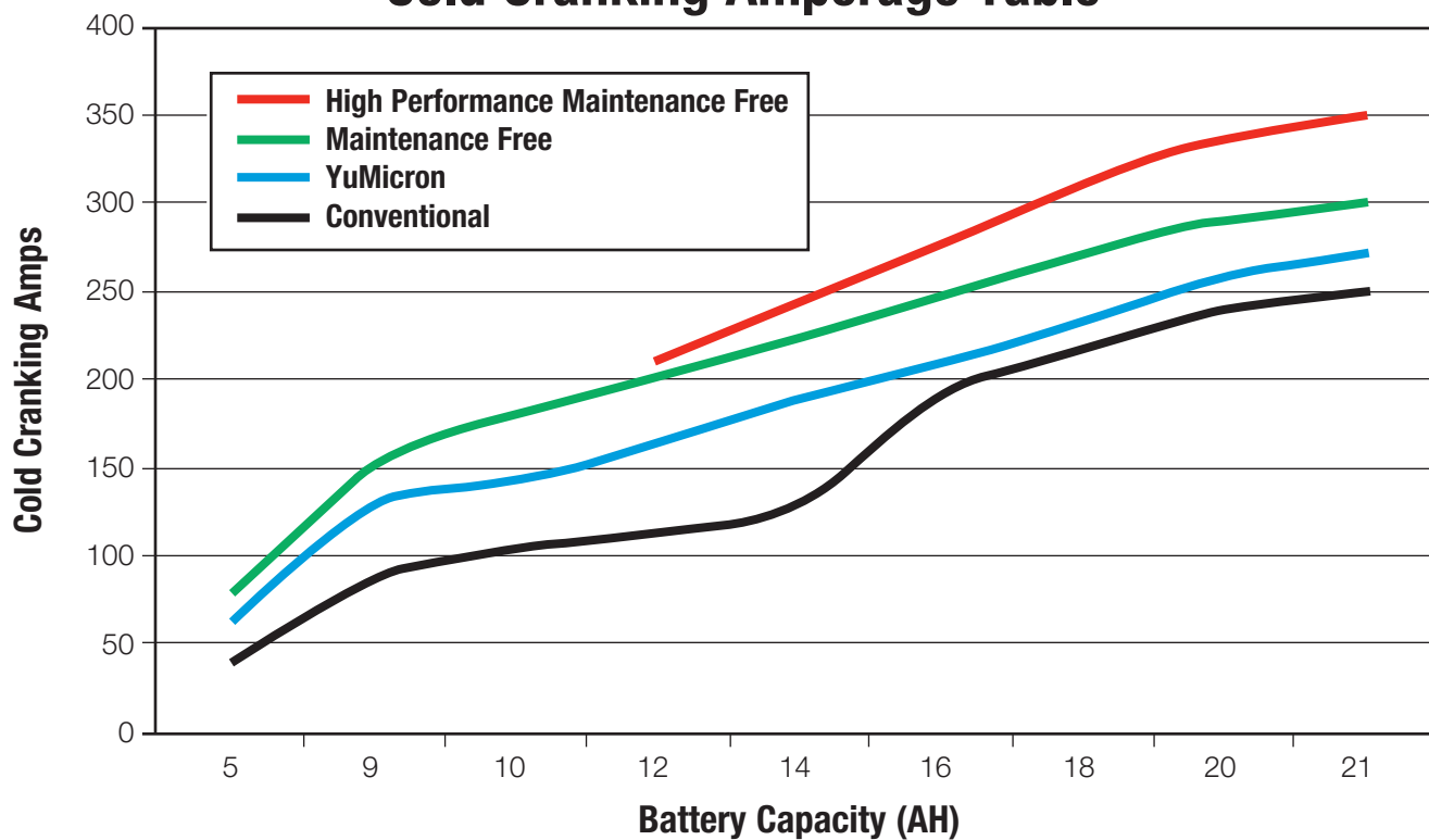
Cold Cranking Amperage Table
