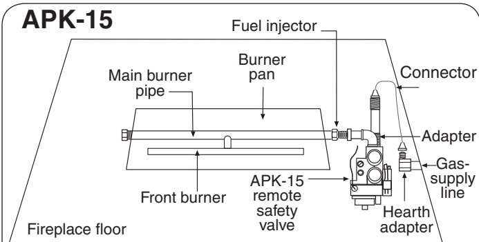
APK-15 Valve
