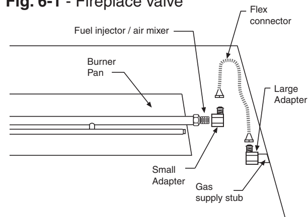
Fig. 6-1 - Fireplace valve
