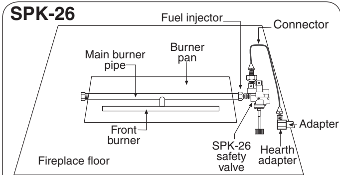
SPK-26 Valve
