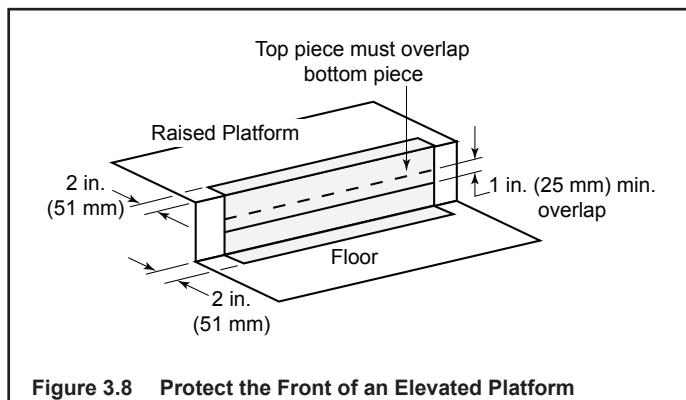
Figure 3.8 Protect the Front of an Elevated Platform
