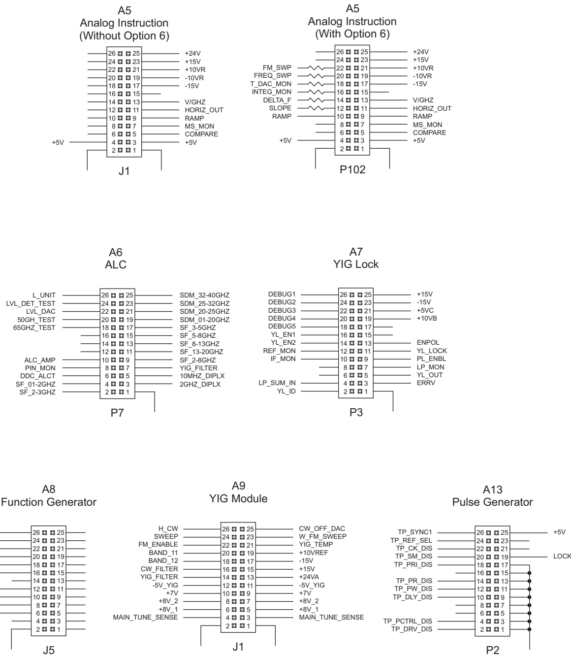
Figure 5-5. PCB Test Point Pinout Diagrams
