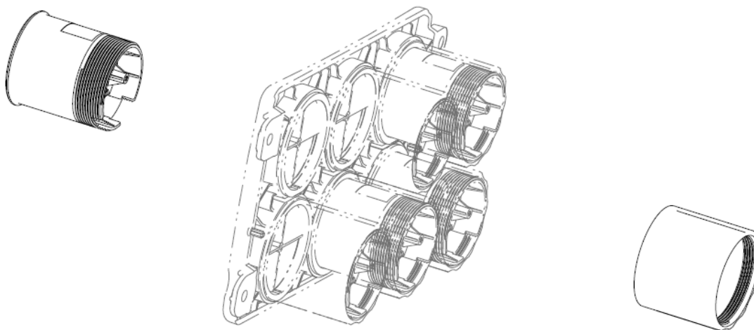
FIGURE 9-43. Gauge Installation
