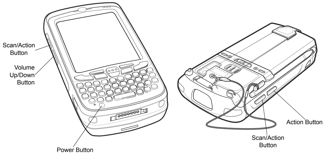
Figure 2-24 Function Buttons
