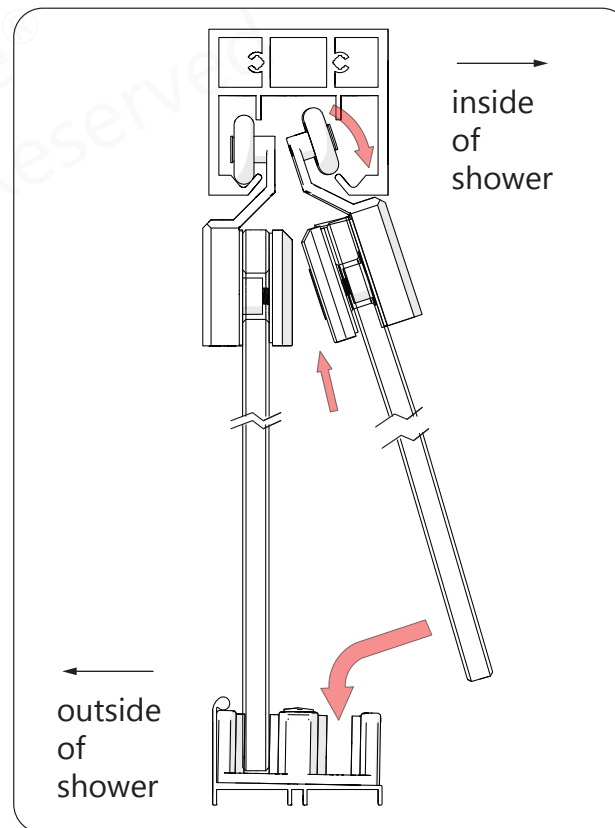
Inside door glass installation
