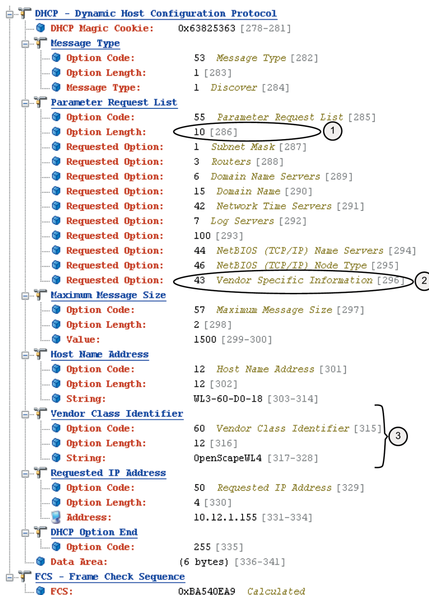
Figure 10: Example of a DHCP Discover Message (Omnipeek Trace)
