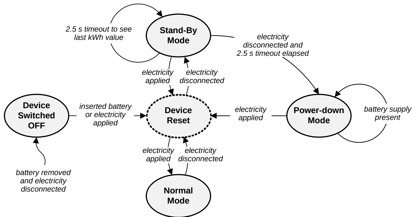
Figure 5-2. Operating modes
