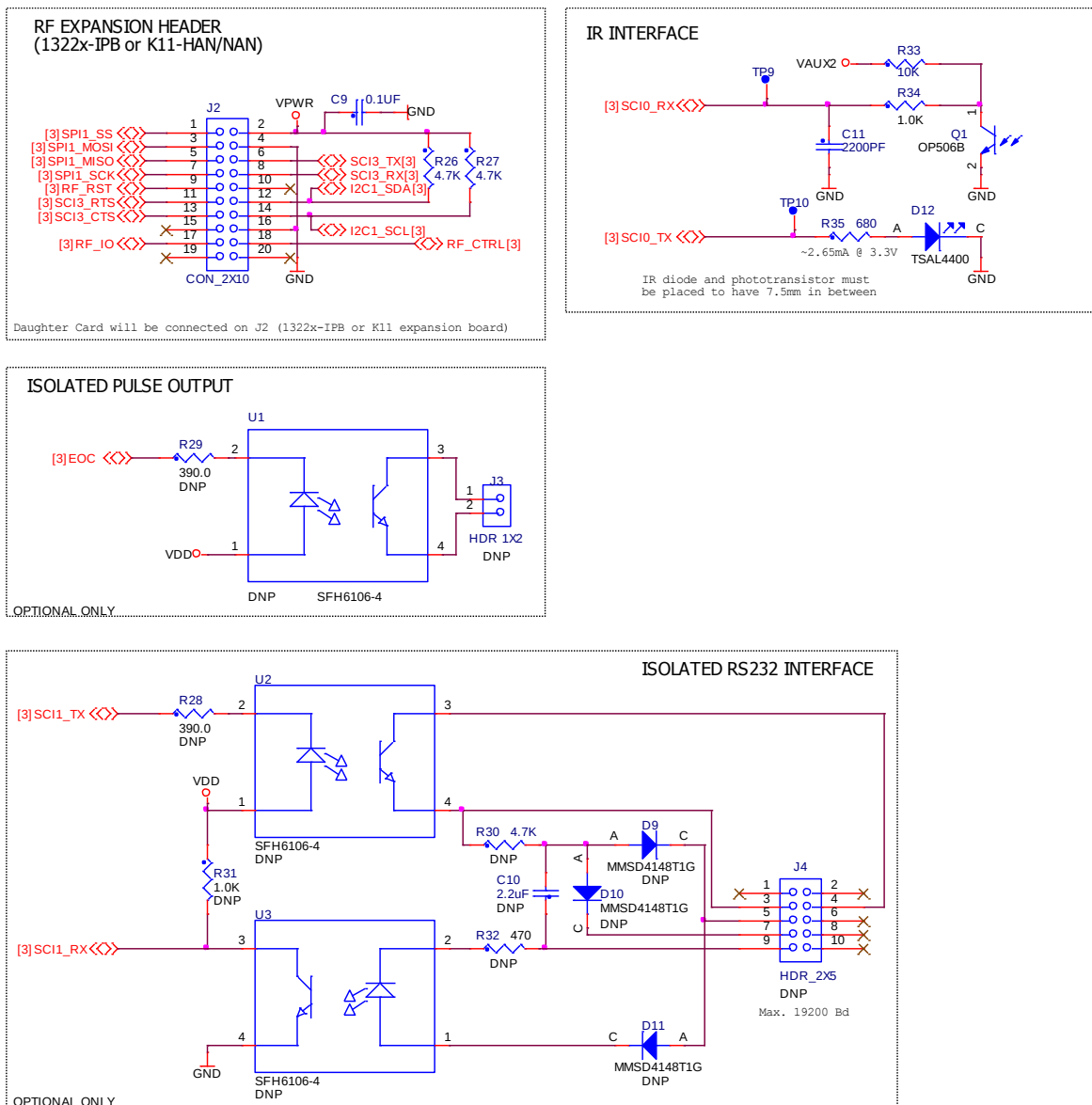
Figure A-3. Schematic diagram of the metering board (sheet 3 of 4 – Interface section)
