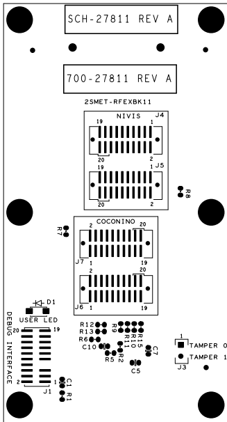
Figure D-2. Bottom side view of the K11 expansion board (not scaled)
