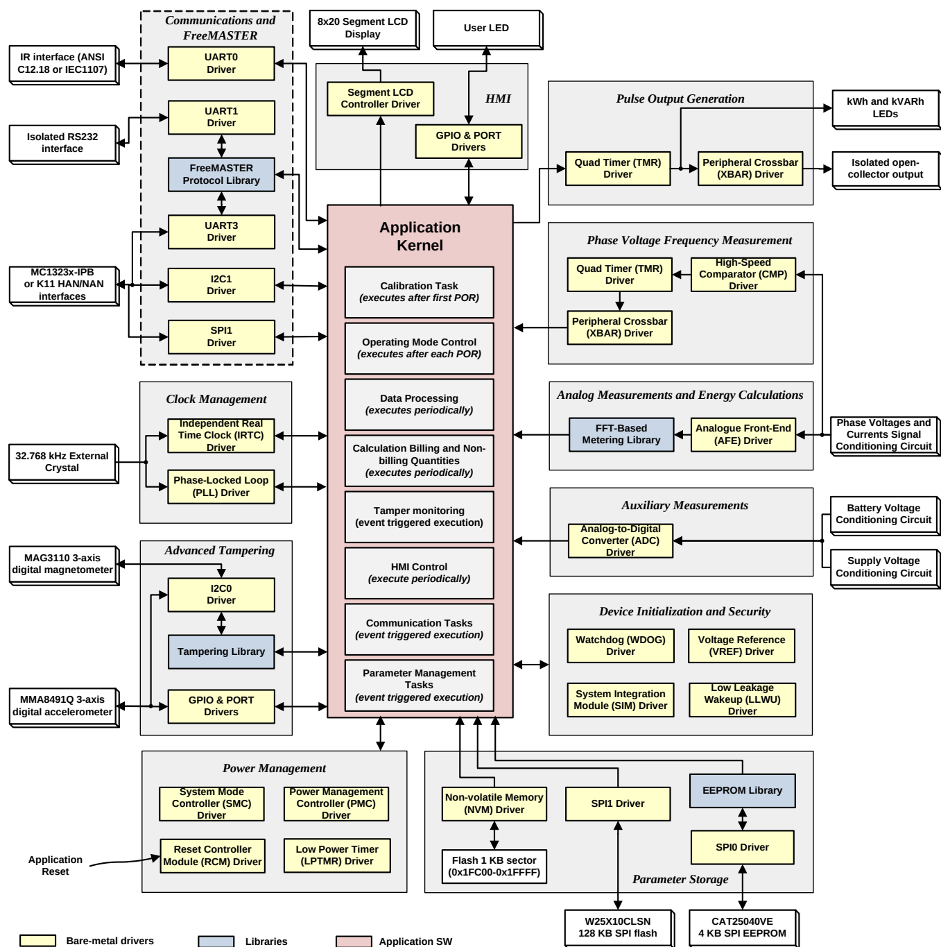
Figure 5-1. Software architecture
