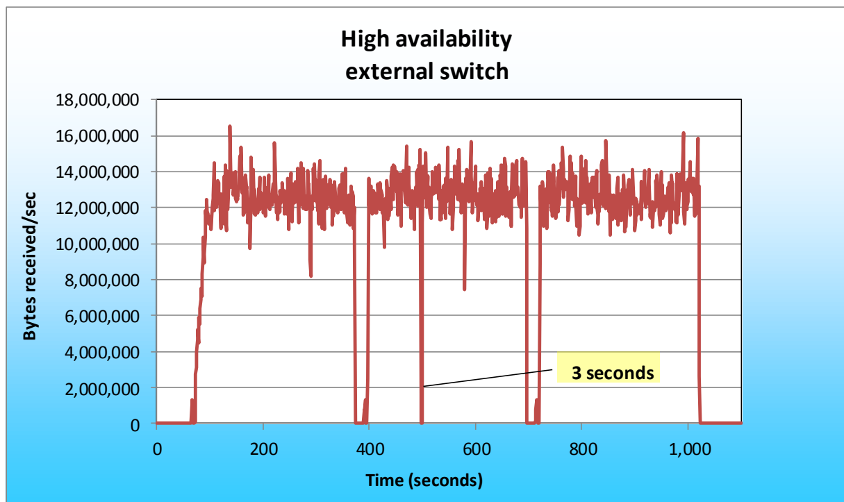
Figure 2: Our external switch high-availability scenario encountered only 3 seconds of downtime.
