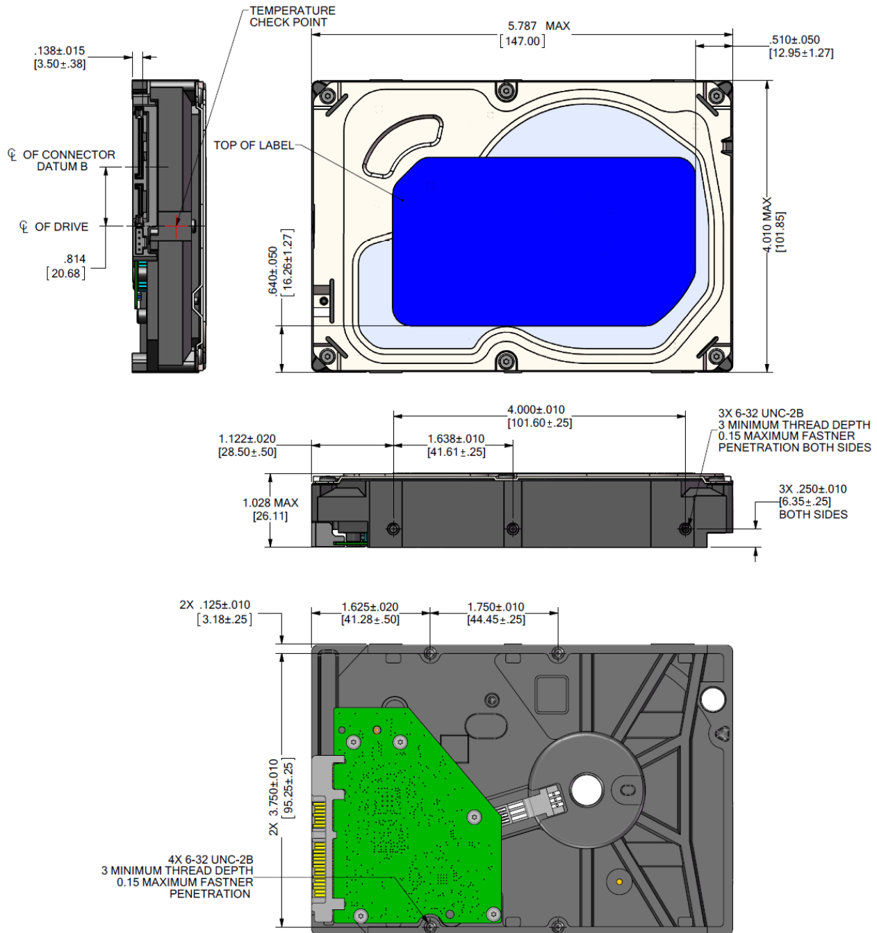
Figure 2 Mounting dimensions (3TB and 4TB)
