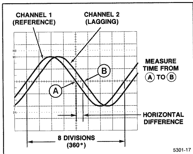
Figure 6-9. Phase difference.
