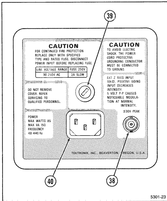
Figure 3-6. Rear Panel.
