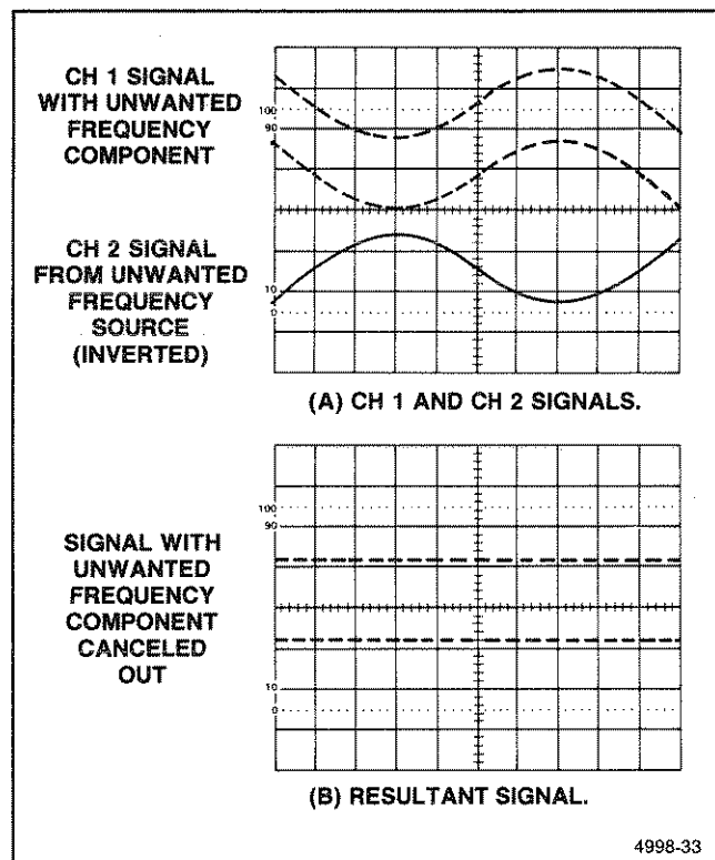
Figure 6-4. Common-mode rejection.
