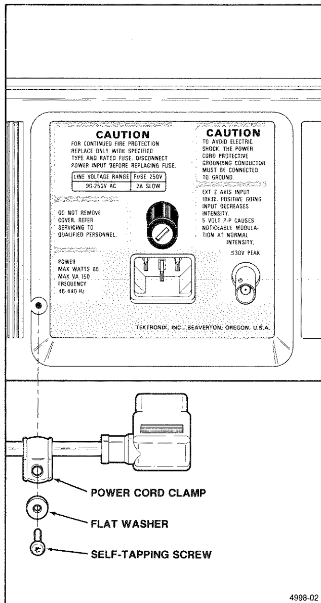
Figure 2-1. Securing the detachable power cord to the instrument.
