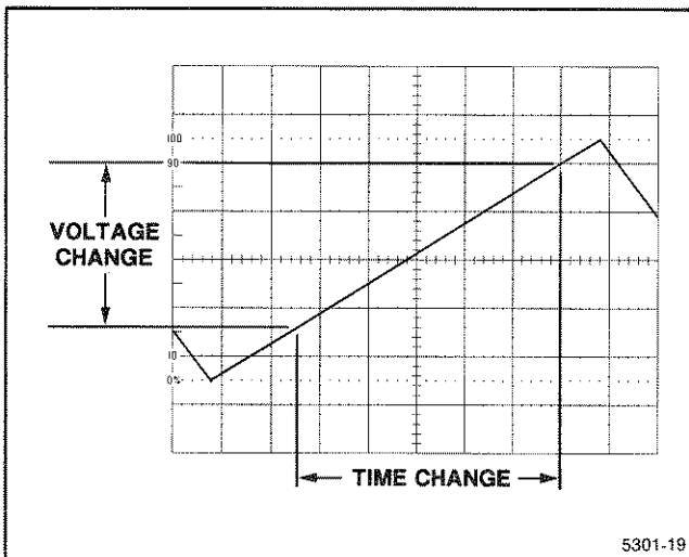
Figure 6-11. Slope.
