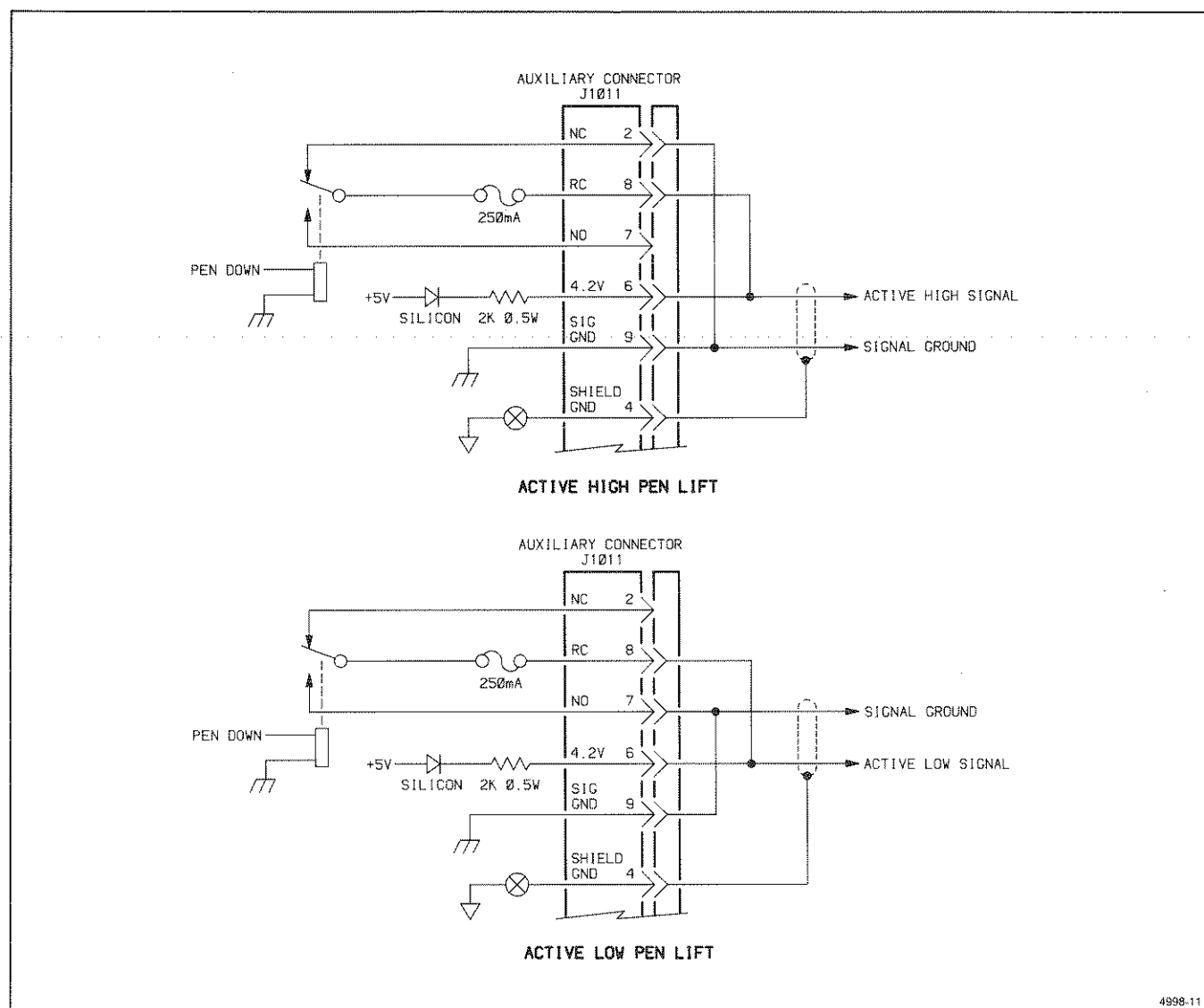
Figure 3-8. X-Y Plotter interfacing.
