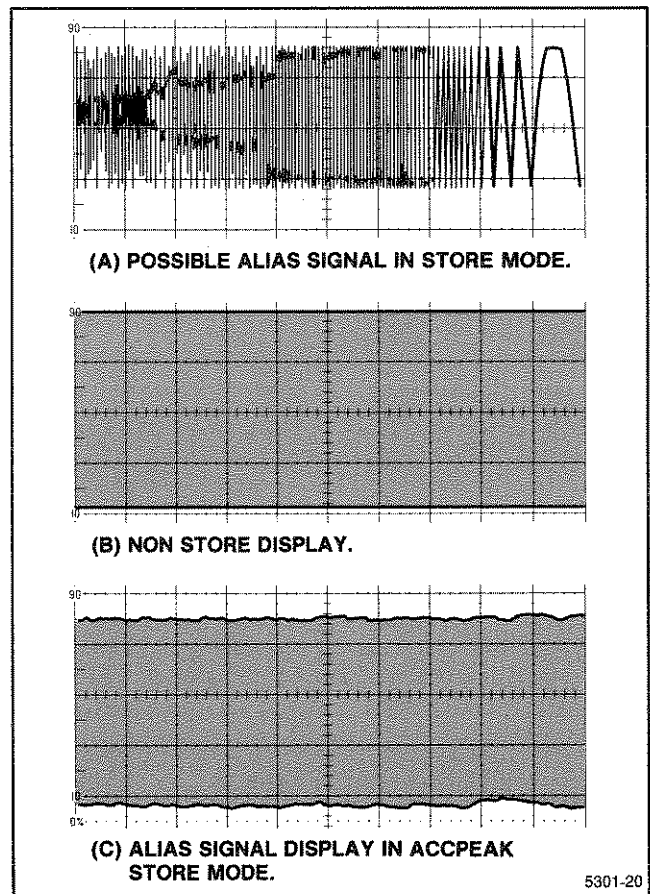
Figure 6-13. Anti-aliasing.
