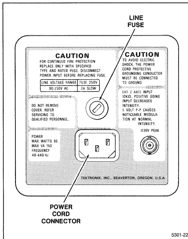
Figure 2-3. Fuse holder and detachable power-cord connector.
