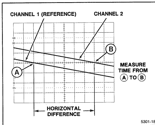
Figure 6-10. High-resolution phase difference.
