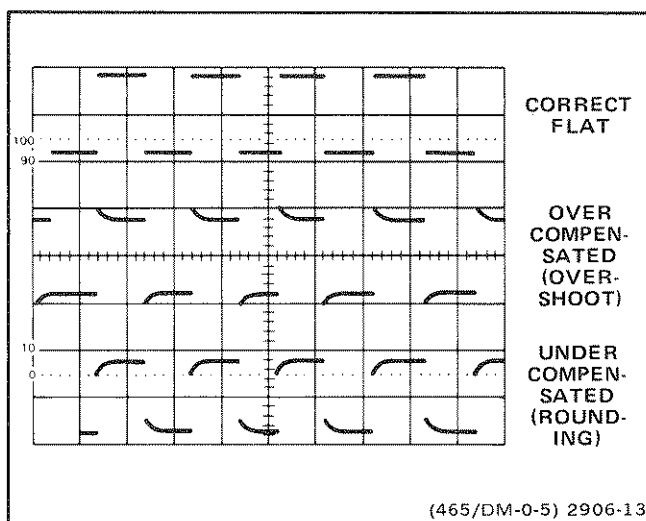
Figure 5-1. Probe compensation.
