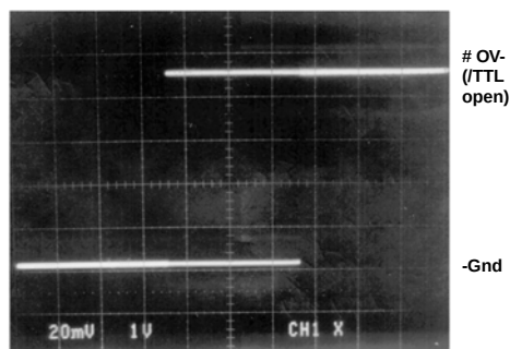
Input/Output Transfer Function - HYS Connected to V
