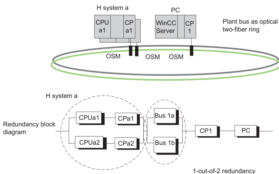
Figure 11-7 Example of redundancy with fault-tolerant system and redundant bus system
