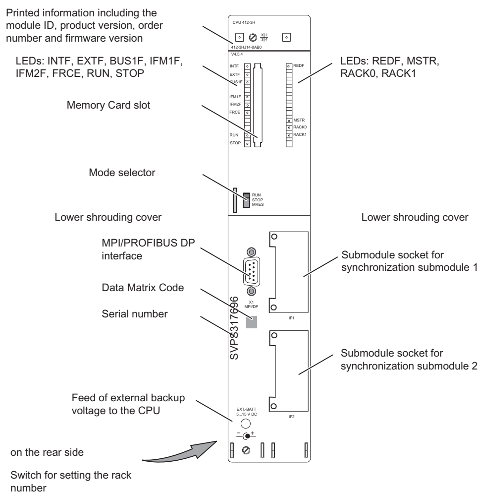
Figure 5-1 Arrangement of the operator controls and display elements on the CPU 412-3H
