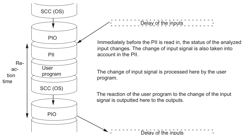
Figure 16-8 Shortest response time
