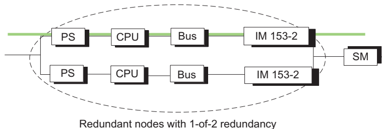
Figure 2-3 Example of redundancy in a network without error
