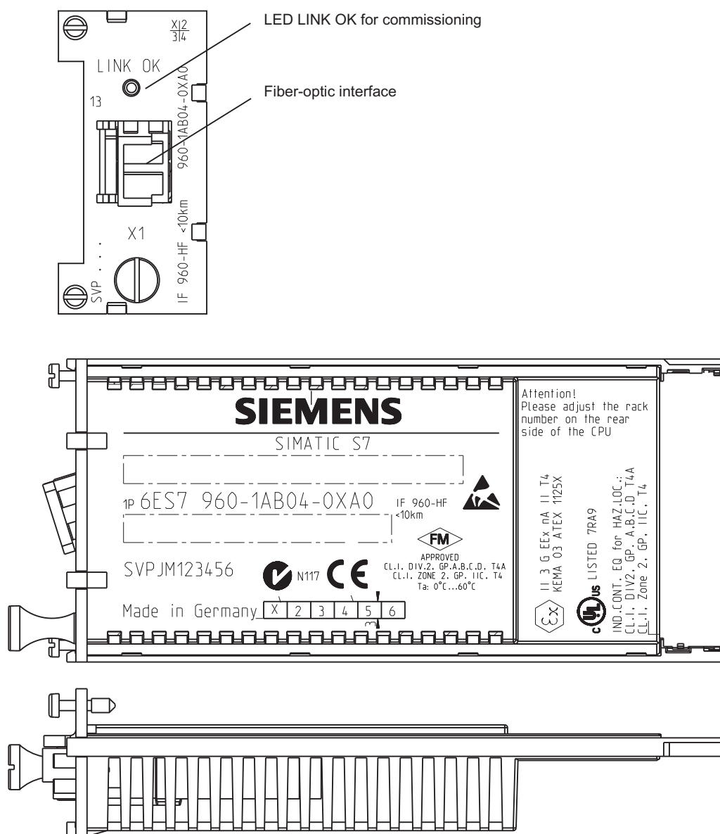
Figure 15-1 Synchronization module
