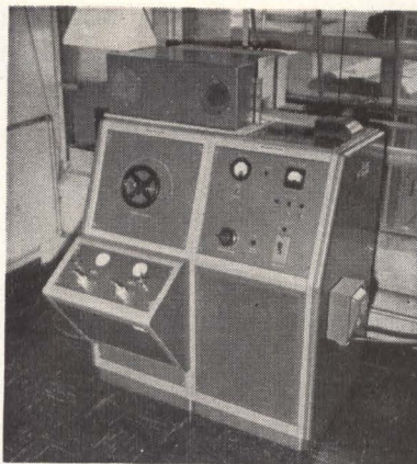
Sintering oven for Teflon sleeving incorporates some modifications to feed mechanism
