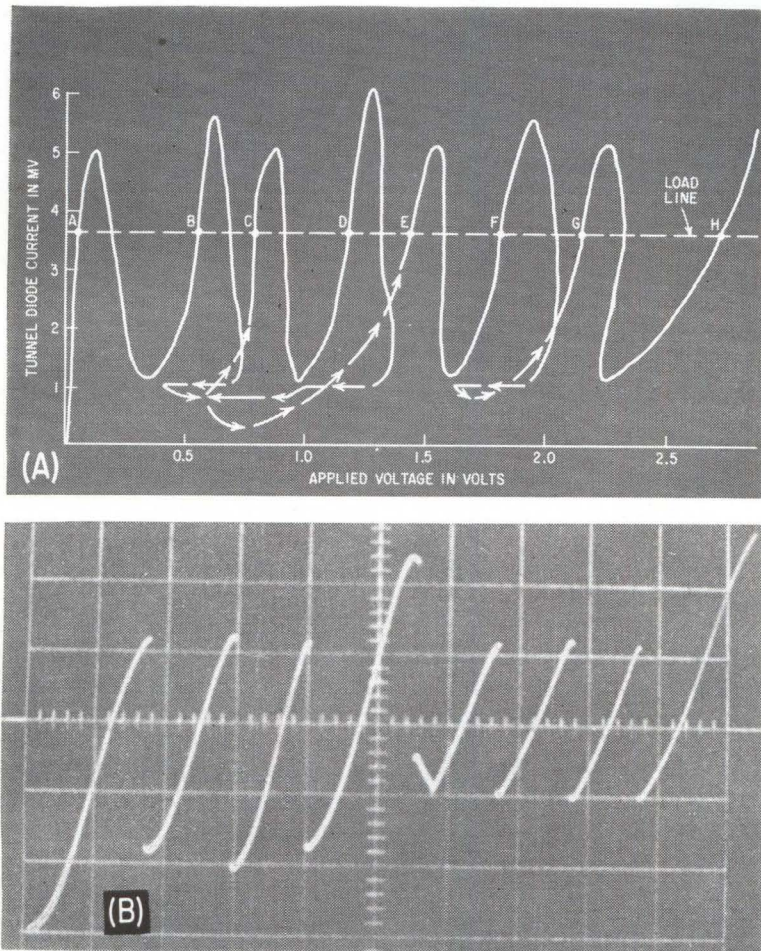
FIG. 2—Composite characteristic of three tunnel diodes connected in series (A) as plotted from theoretical values, and (B) an oscillogram of three commercial tunnel diodes in series
