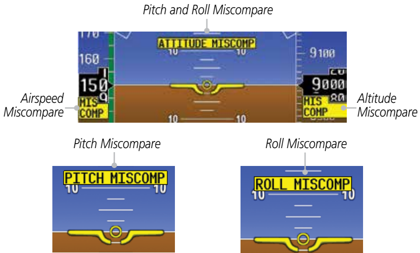
Figure 2-40 Miscompare Annunciations
