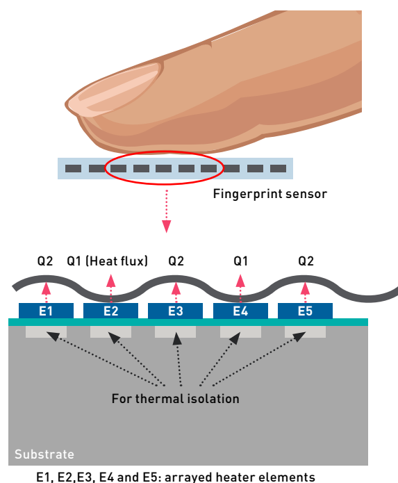
Figure 30. Principle of active thermal fingerprint detection
