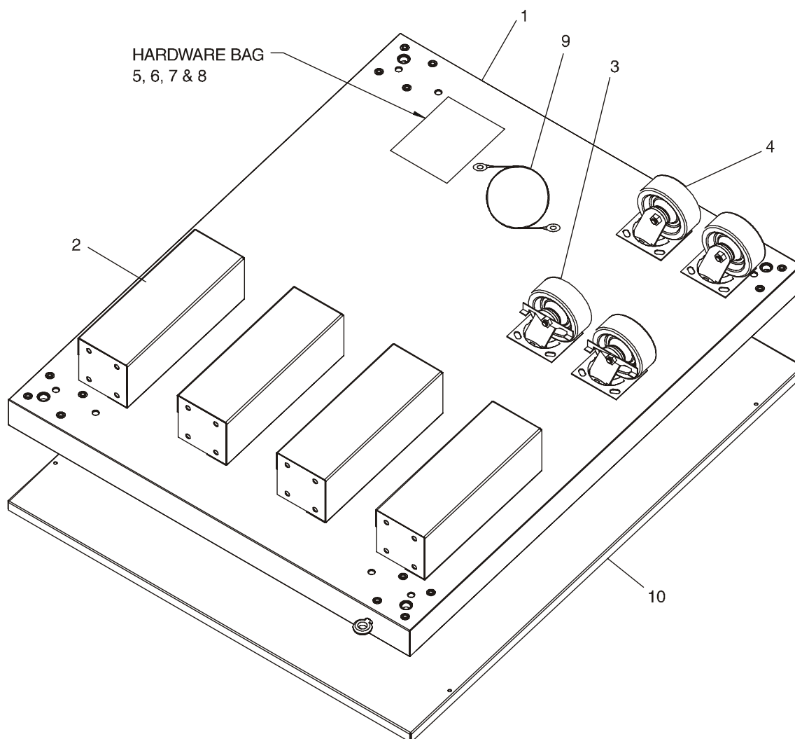
Figure 2-2. Model PS540 Single Oven Option Base with Legs and Top
