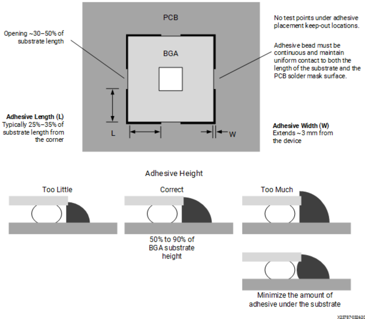
Figure 37: Edge Bonding Adhesive Placement Parameters
