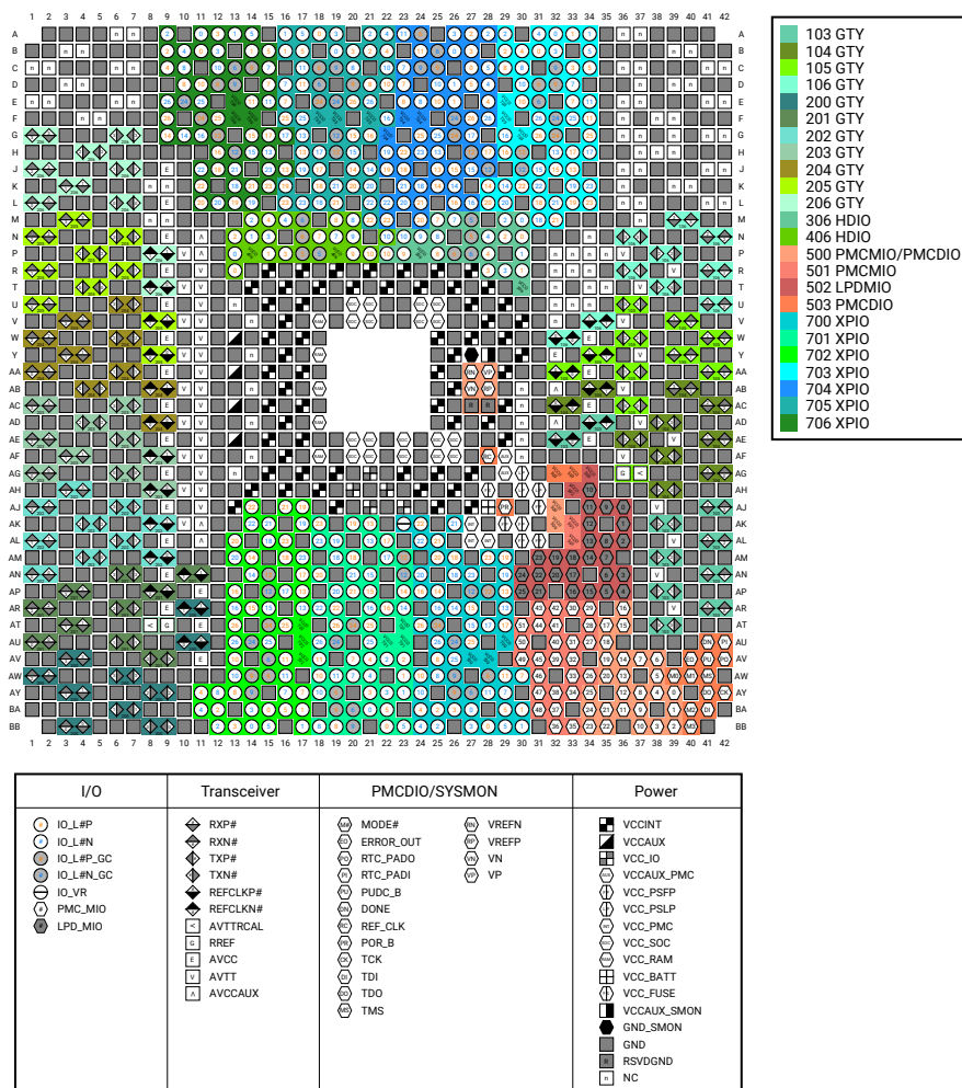
Figure 16: VFVC1760 Package—VM1802 Device Diagram
