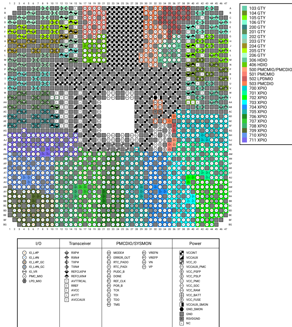
Figure 21: VSVA2197 Package—VC1902 Device Diagram
