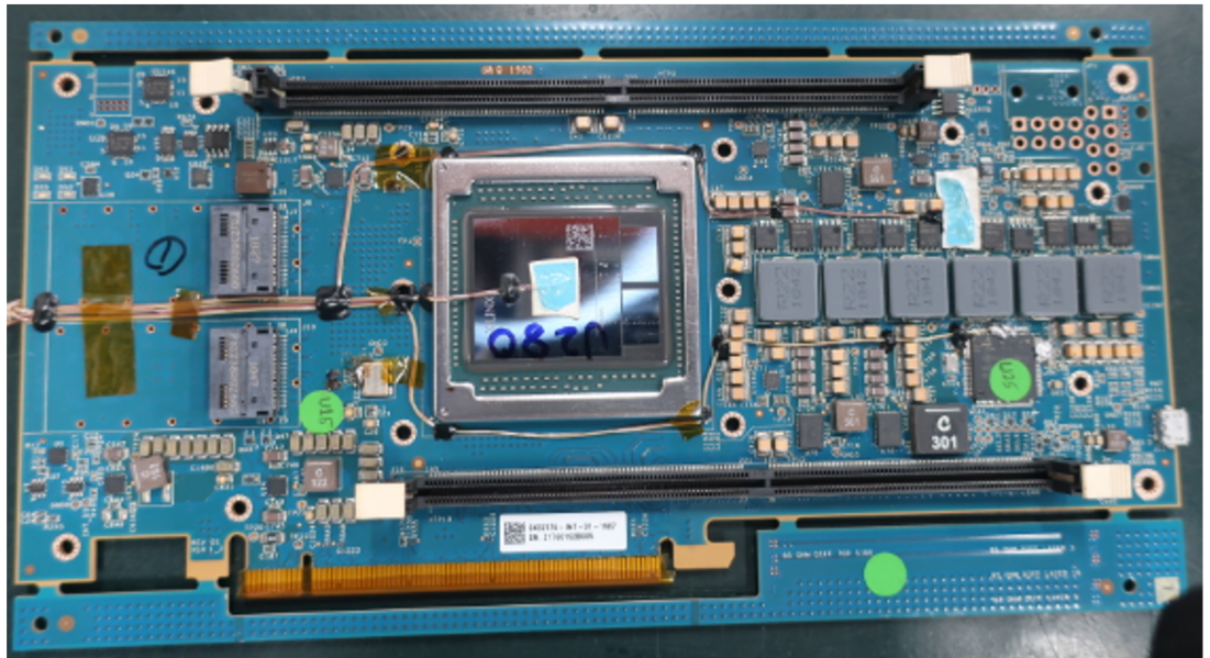
Figure 30: Thermocouple Top
