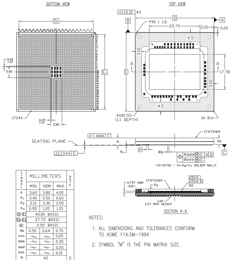
Figure 25: Package Dimensions for VSVD1760 (VC1802, VC1902, and VM1802)
