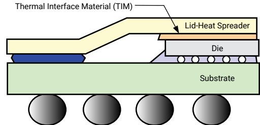
Figure 38: Heat Spreader with Thermal Interface Material
