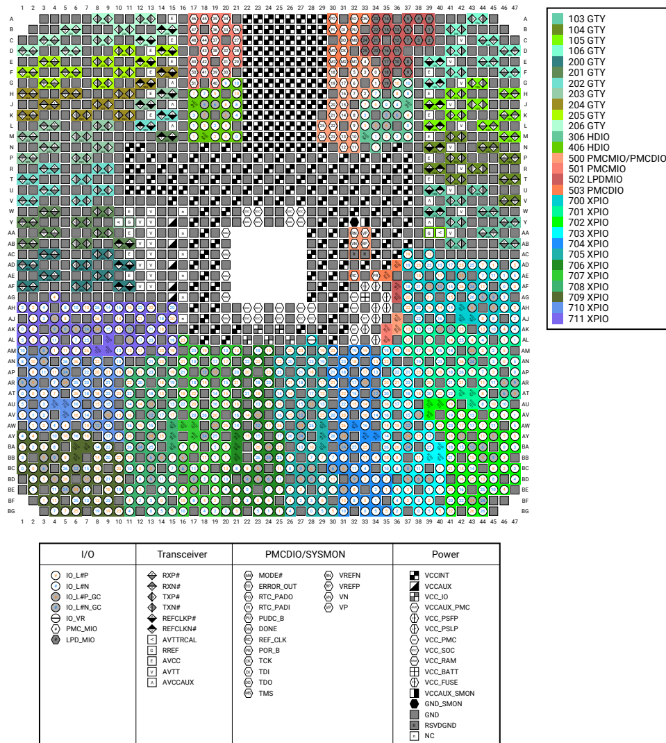
Figure 22: VSVA2197 Package—VM1802 Device Diagram
