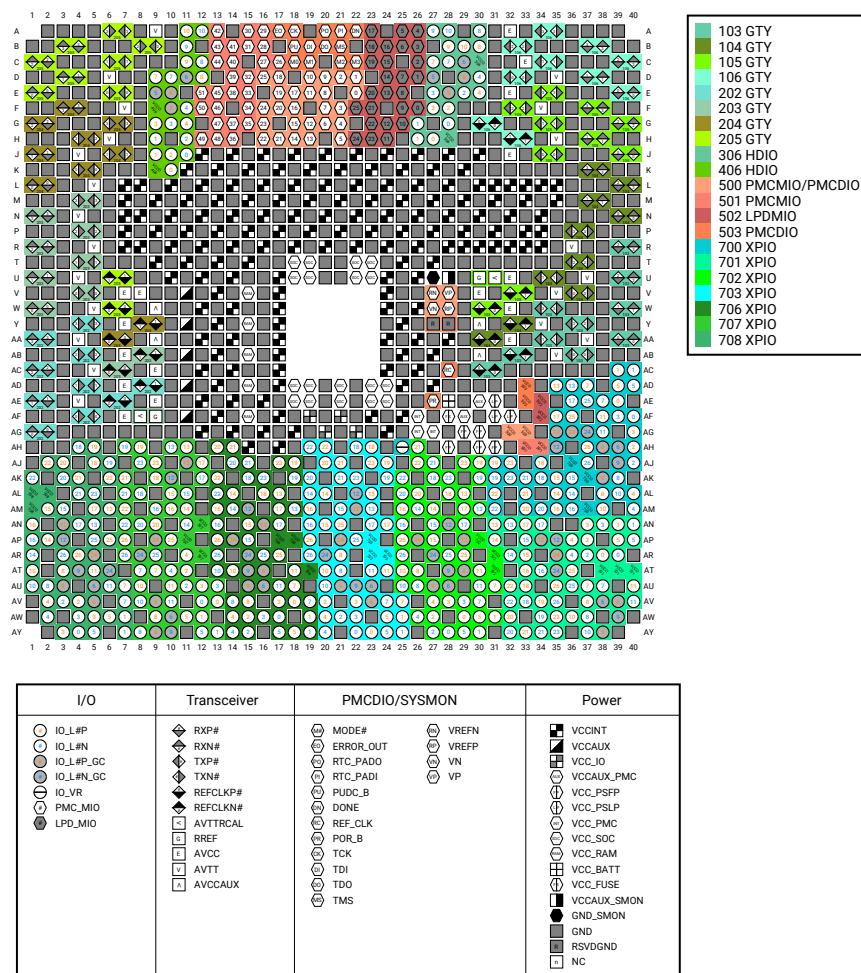
Figure 14: VIVA1596 Package—VC1802 Device Diagram
