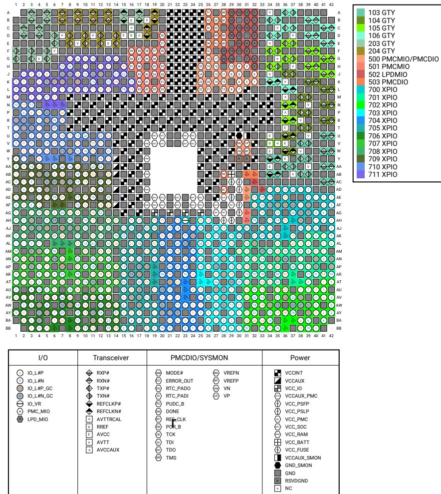
Figure 18: OLD VSVD1760 Package—VC1902 Device Diagram
