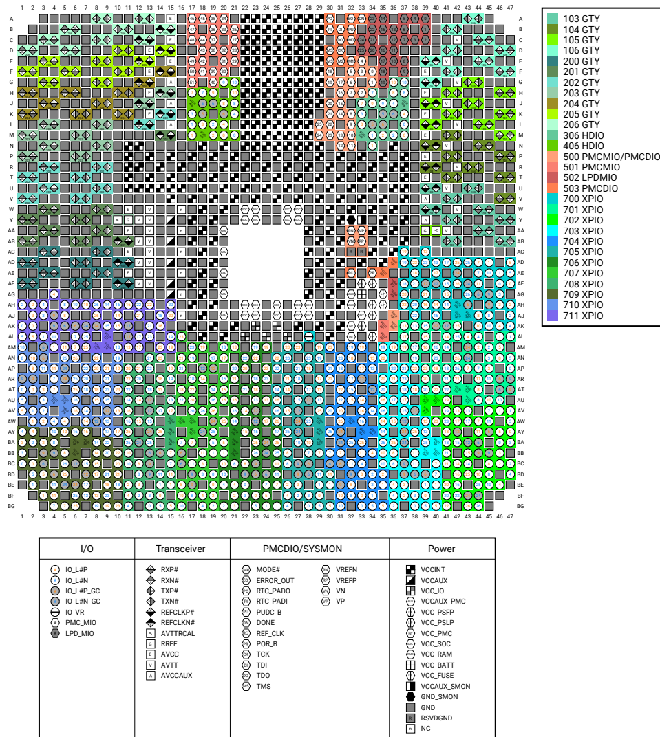
Figure 20: VSVA2197 Package—VC1902 Device Diagram
