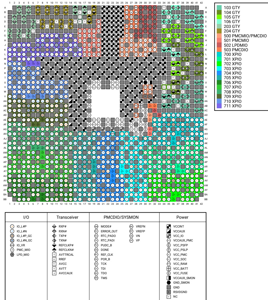
Figure 19: VSVD1760 Package—VM1802 Device Diagram
