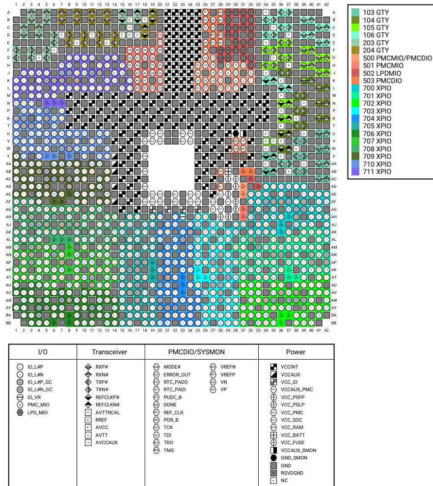
Figure 17: VSVD1760 Package—VC1802 Device Diagram
