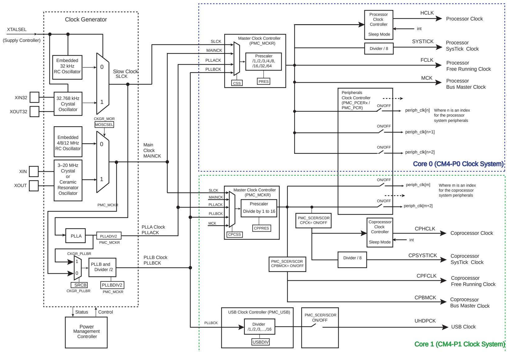
General Clock Block Diagram (USB-equipped devices)
