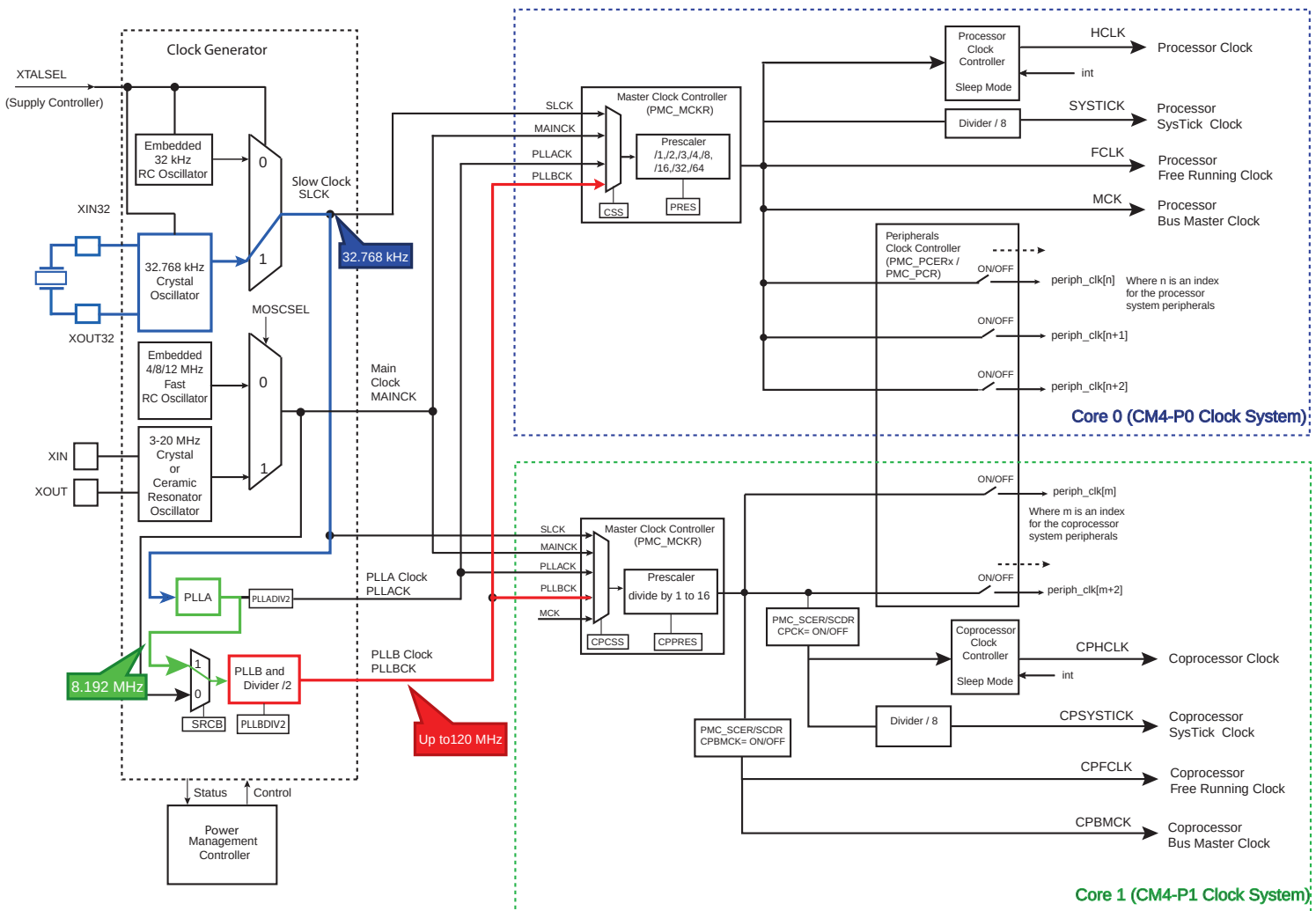
SAM4C16/8/4 Global Clock System
