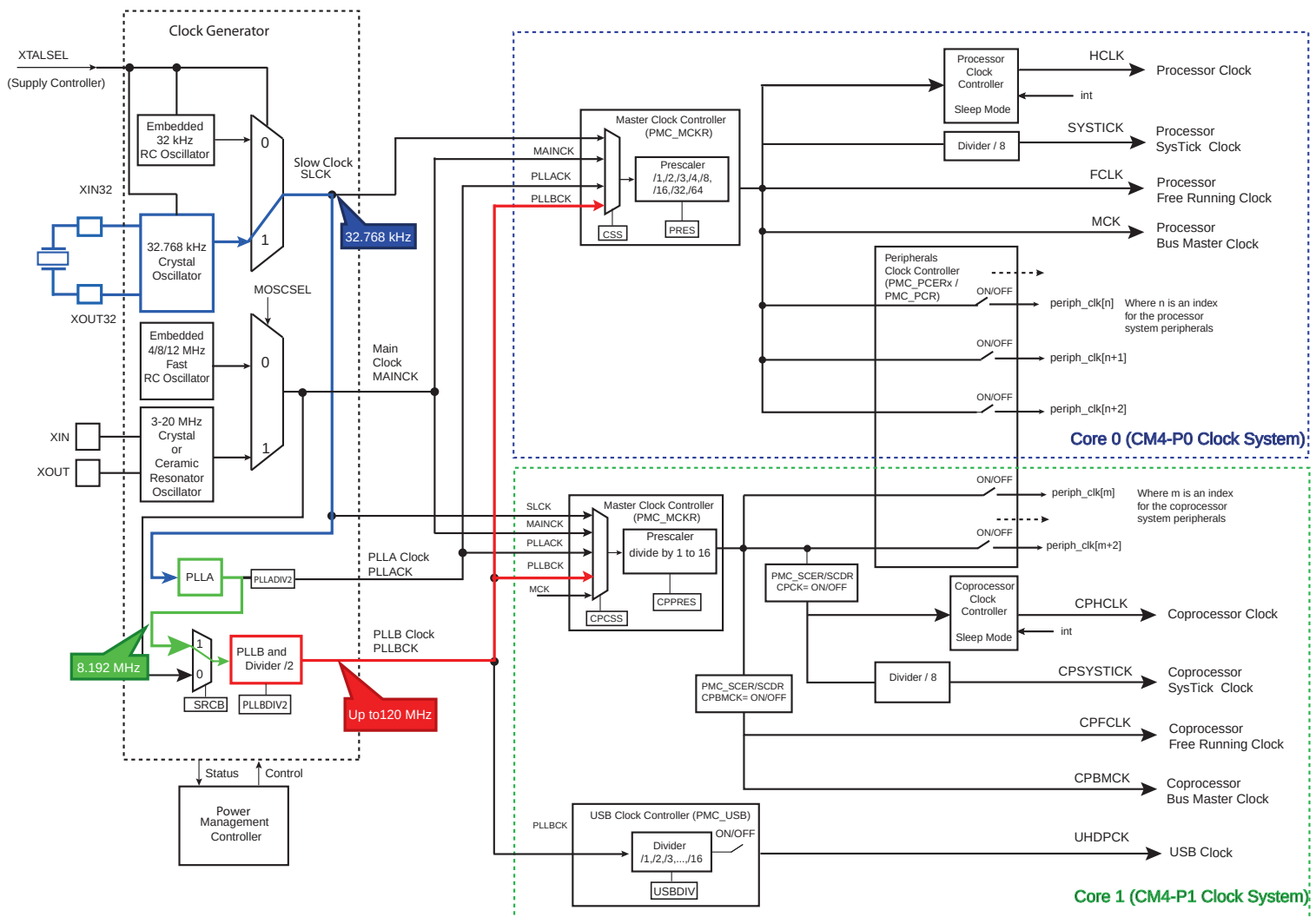
SAM4C32 Global Clock System
