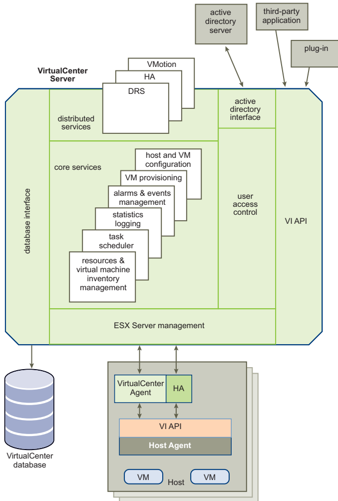
Figure 12. VirtualCenter Server Components
