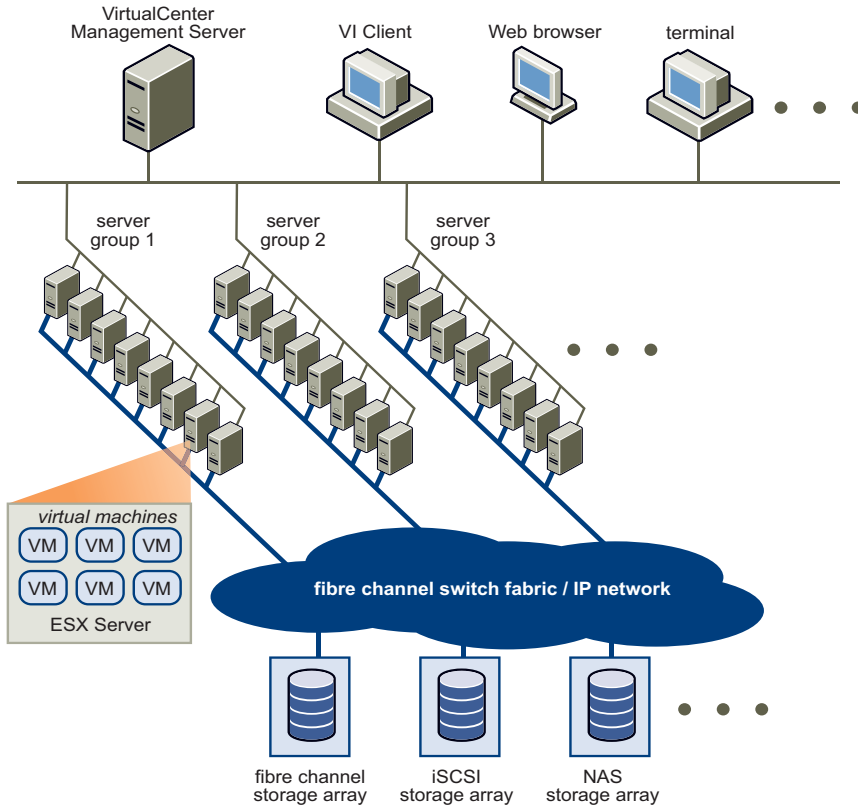
Figure 2. VMware Infrastructure Datacenter Physical Topology
