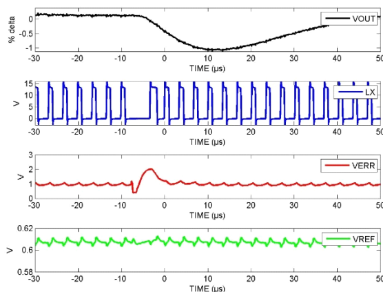
FIGURE 4. Worst case SET captured for each of the three units tested at P_{VIN} = 13.2\text{V} , V_{OUT} = 3.3\text{V} , I_{OUT} = 3\text{A} , frequency = 300kHz internal and LET = 86 \text{ MeV} \cdot \text{cm}^2/\text{mg} . Worst case SET was -1.2% or 40mV.
