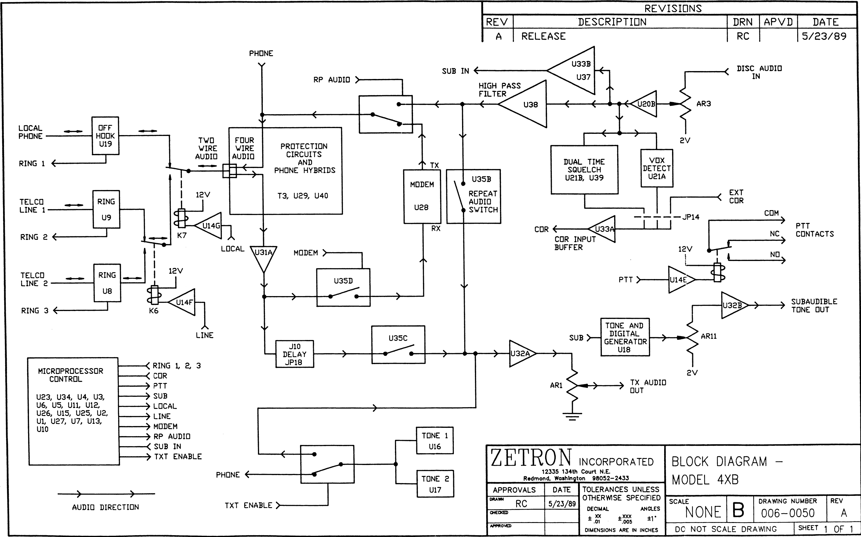
MODEL 4XB BLOCK DIAGRAM (006-0050A)
