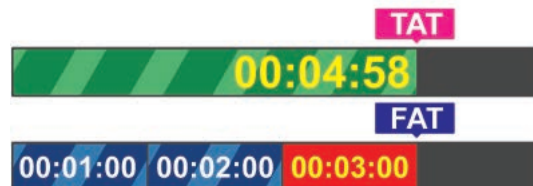
FAT storage loses nearly 1 minute of video after power shutoff.
