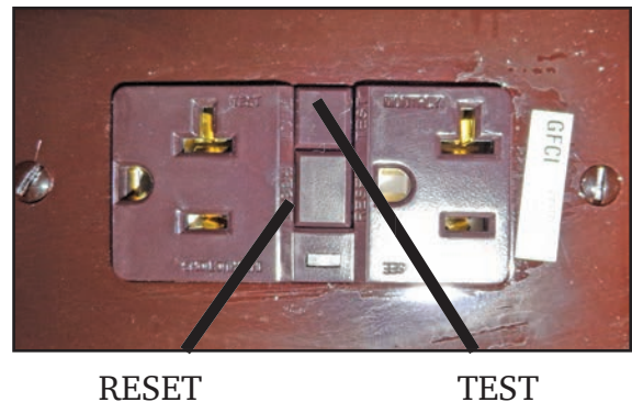
Figure 9-3: GFCI receptacle
