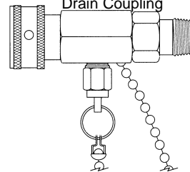
FD15 Series – page 292 Oil Sampling Valve
