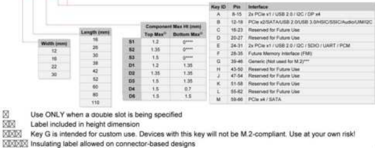
Figure 6-3 M.2 interface model
