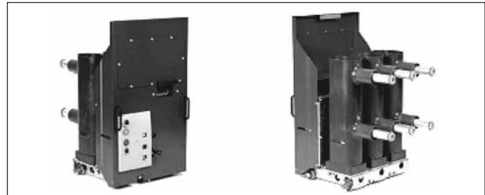
Figure 10. Front and Back Views of a Typical IEC MV Vacuum Circuit Breaker
