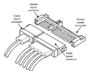
Figure 1 Attaching SATA cabling
