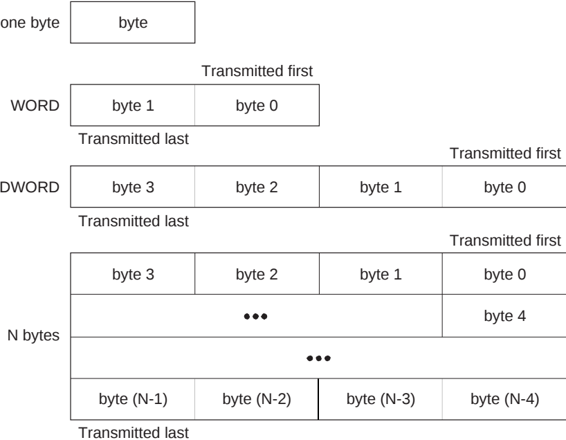
Figure 3-2 Byte Ordering
