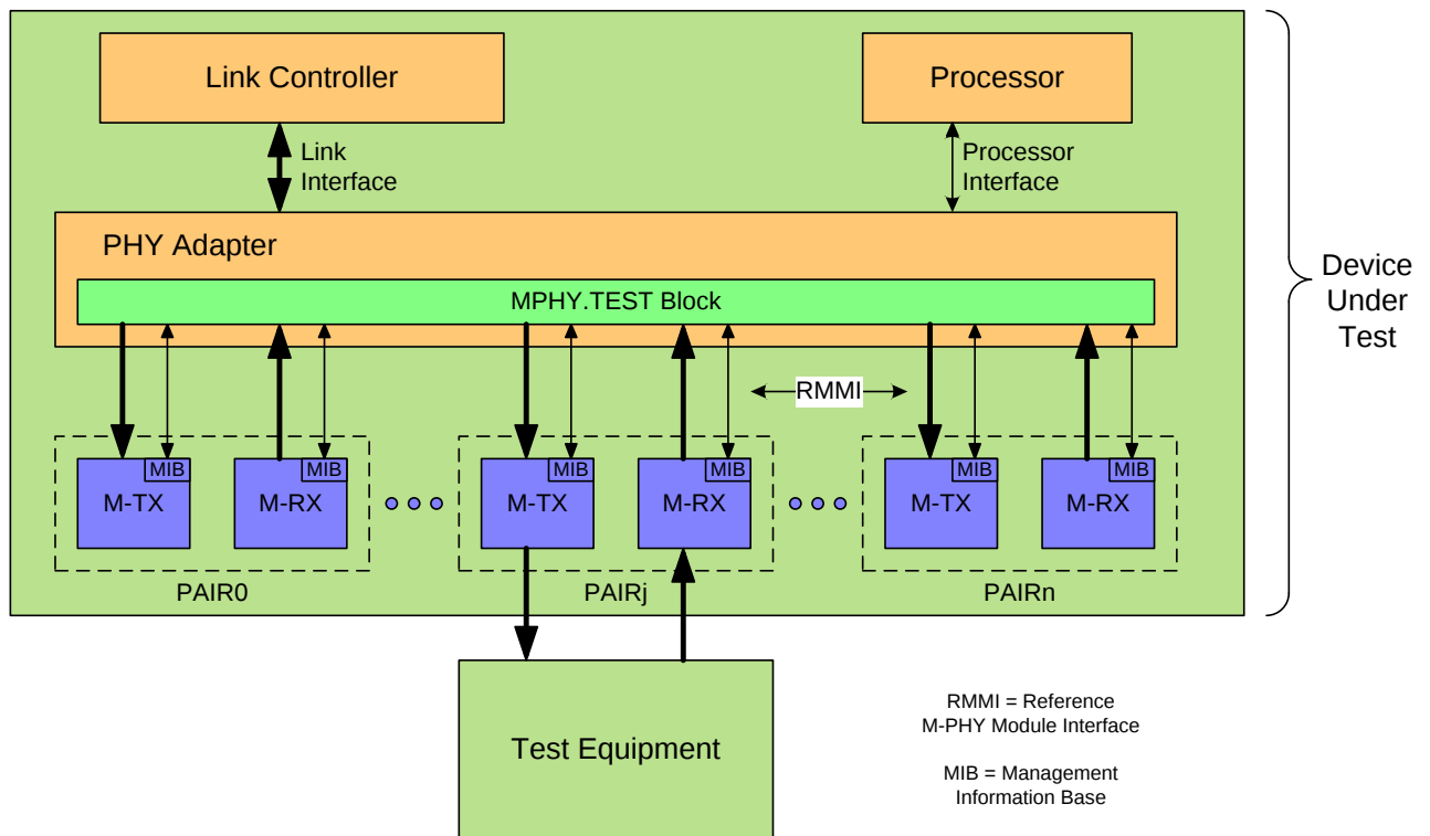
Figure 6-1 MPHY.TEST Overview
