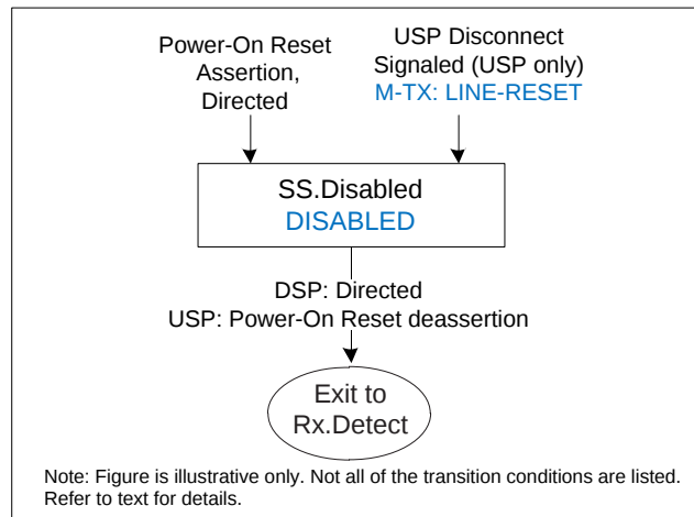
Figure 3-8 SS.Disabled state
