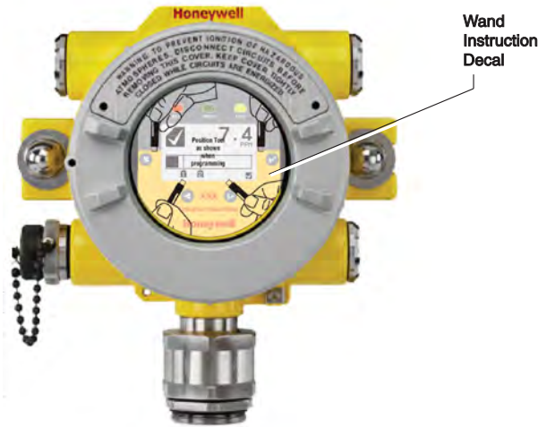
Figure 10. Operation decal
