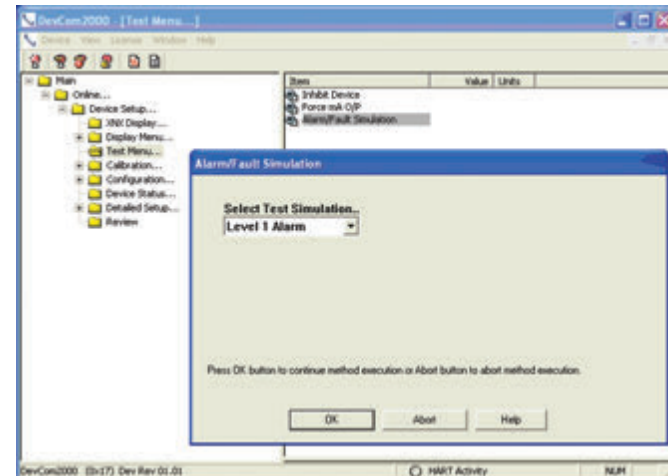
Figure 244. Alarm Simulation
