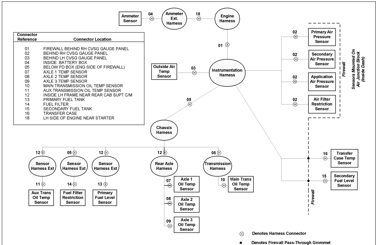
FIGURE 6-5. Instrumentation Harness Interface Diagram
