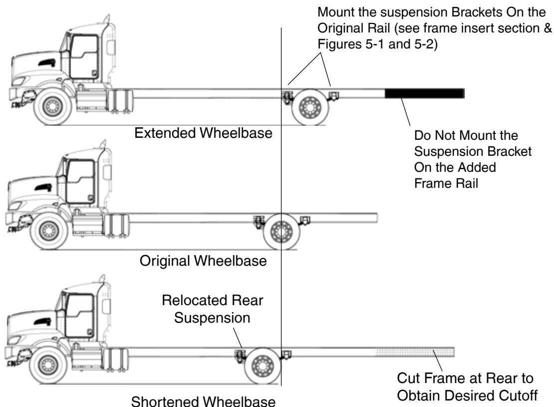
FIGURE 5-3. Comparison of Original, Shortened, and Extended Wheelbases.
