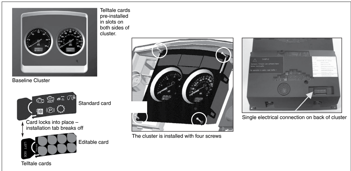
FIGURE 6-2. Instrument Cluster Componentry.
