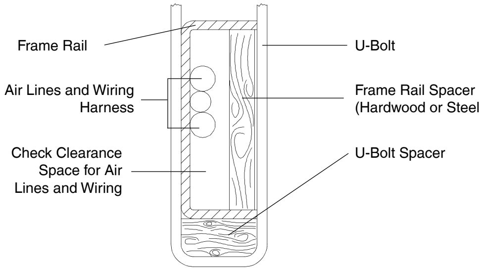
FIGURE 4-8. Clearance Space for Air Lines and Cables
