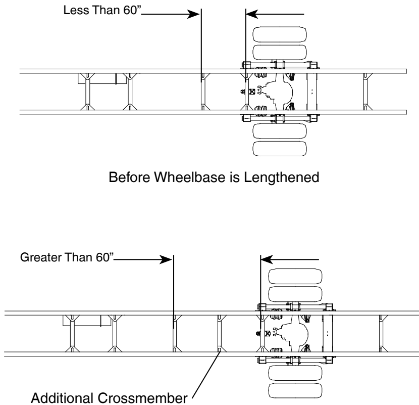
FIGURE 5-4. Crossmember Added When Distance Exceeds 60 Inches (1524 mm)
