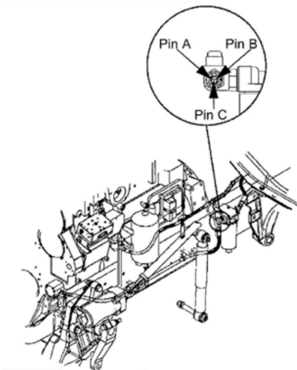
FIGURE 6-6. Firewall Air Junction Block
