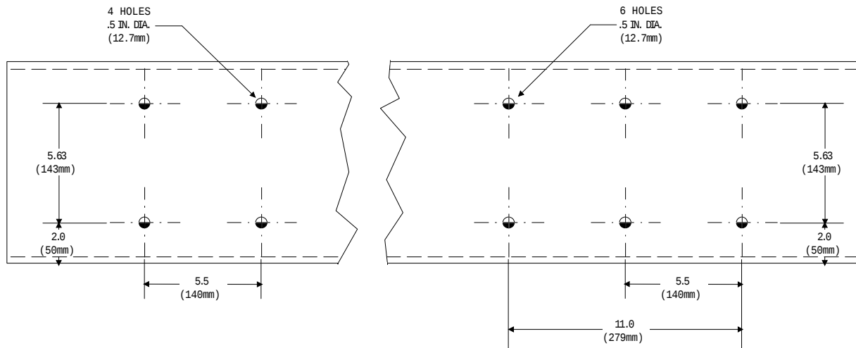
FIGURE 4-6. Crossmember-Gusset Hole Pattern Requirements. [inch (mm)]
