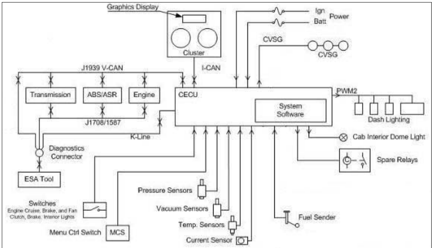
FIGURE 6-4. Multiplexed Instrumentation Block Diagram.
