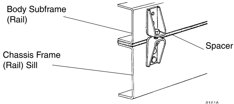
FIGURE 4-3. Spacer Between Frame Sill and Body Rail - Rubber or Plastic
