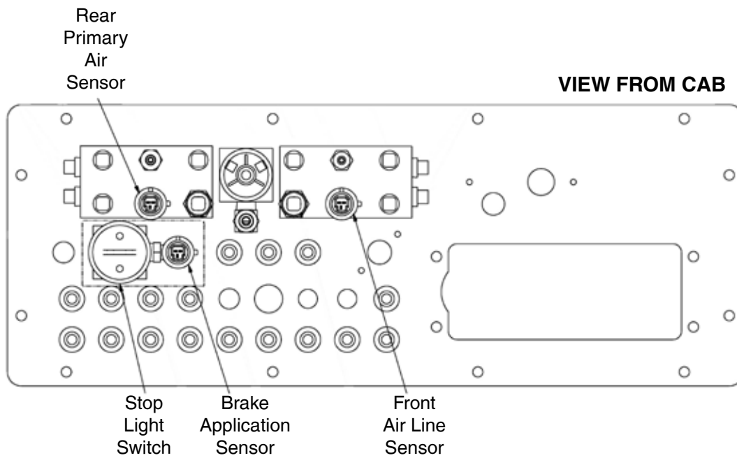
FIGURE 6-6. Firewall Air Junction Block
