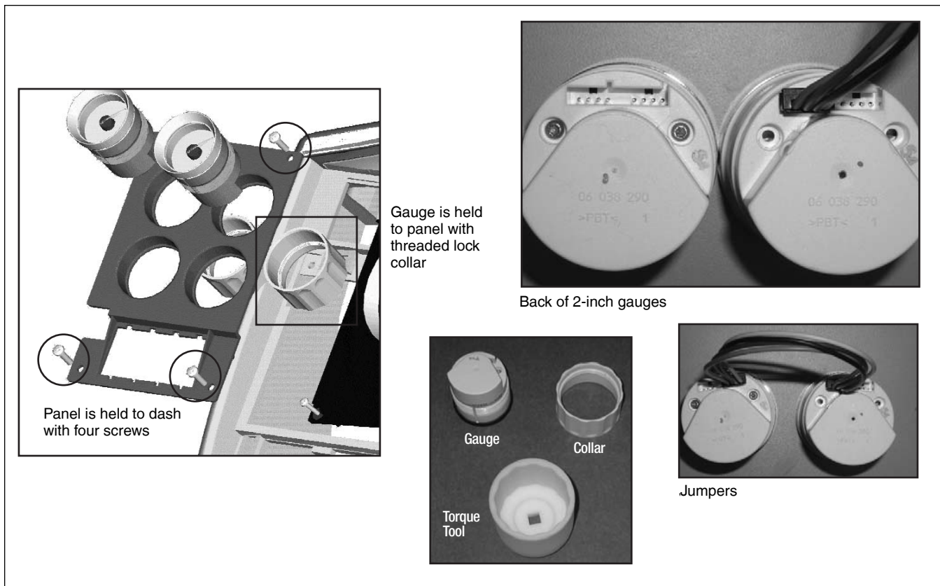
FIGURE 6-3. CVSG Gauges.
