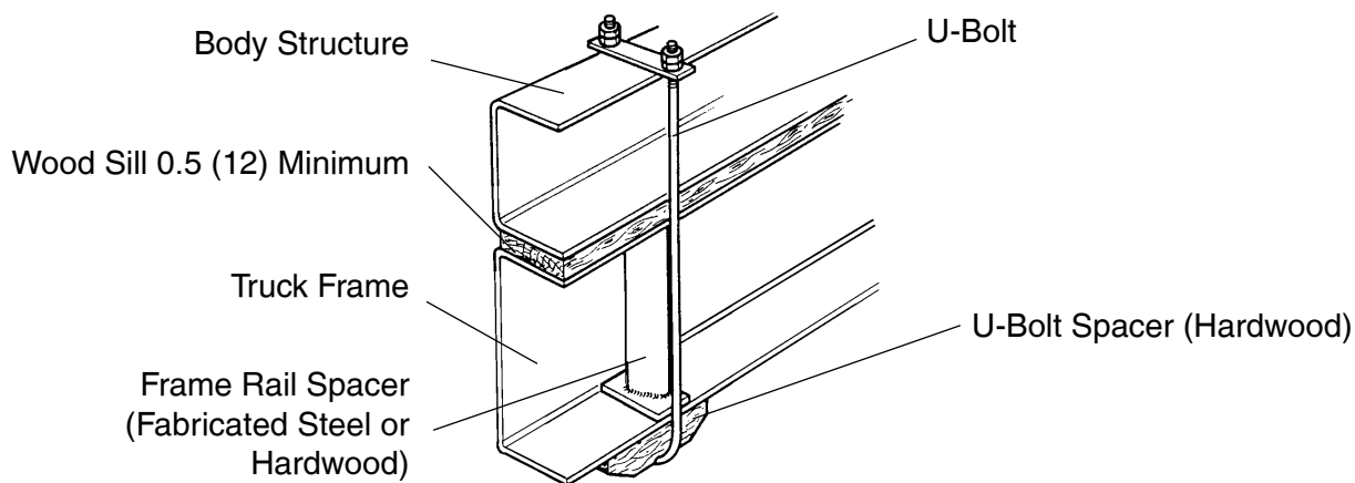
FIGURE 4-7. Acceptable U-Bolt Mounting with Wood and Fabricated Spacers [inch (mm)]
