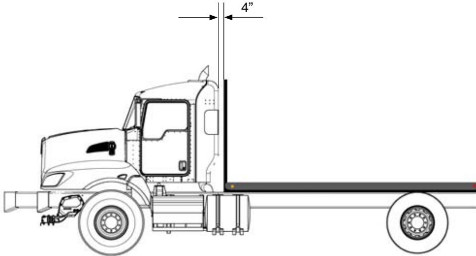
FIGURE 4-2. Minimum Back of Cab Clearance
