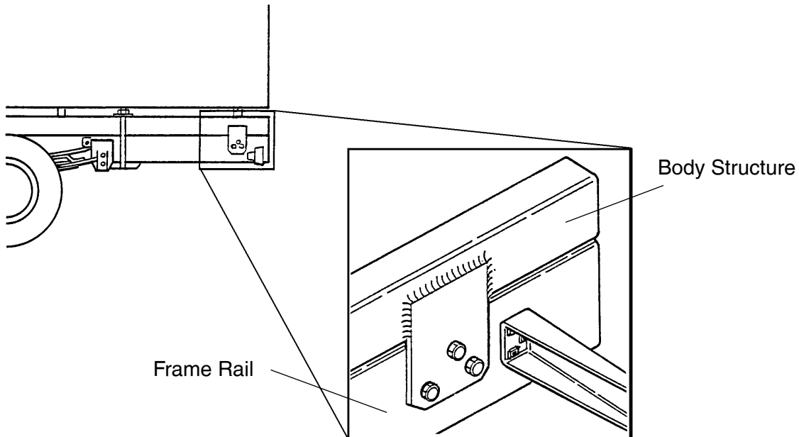
FIGURE 4-9. Example of Fishplate Bracket at Rear End of Body, used with U-Bolts
