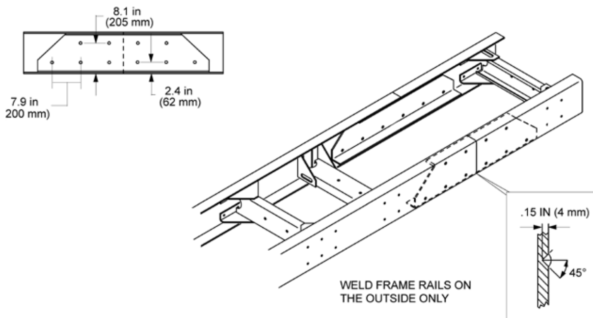
FIGURE 5-1. Detail of Frame Extension and Joint Welding
