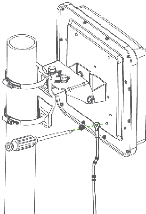
Figure 10 Grounding Example
