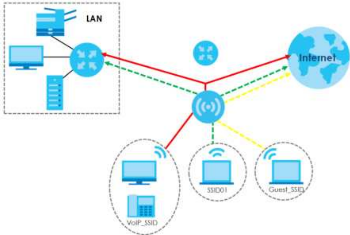
Figure 1 Multiple BSSs
