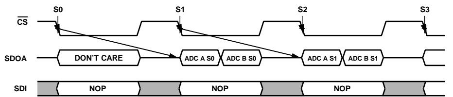
Figure 42. Reading Conversion Results: 1-Wire Mode
