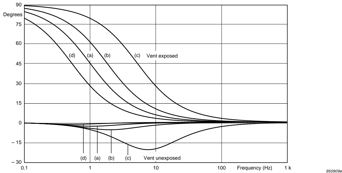
Fig. 2.9 The phase of the low frequency microphone response is influenced by the ambient pressure. The calculated responses shown are valid for a microphone which has 10% air-stiffness at nominal ambient pressure (101.3 kPa): a) 1 bar; b) 2 bar; c) 10 bar; d) 0.5 bar
