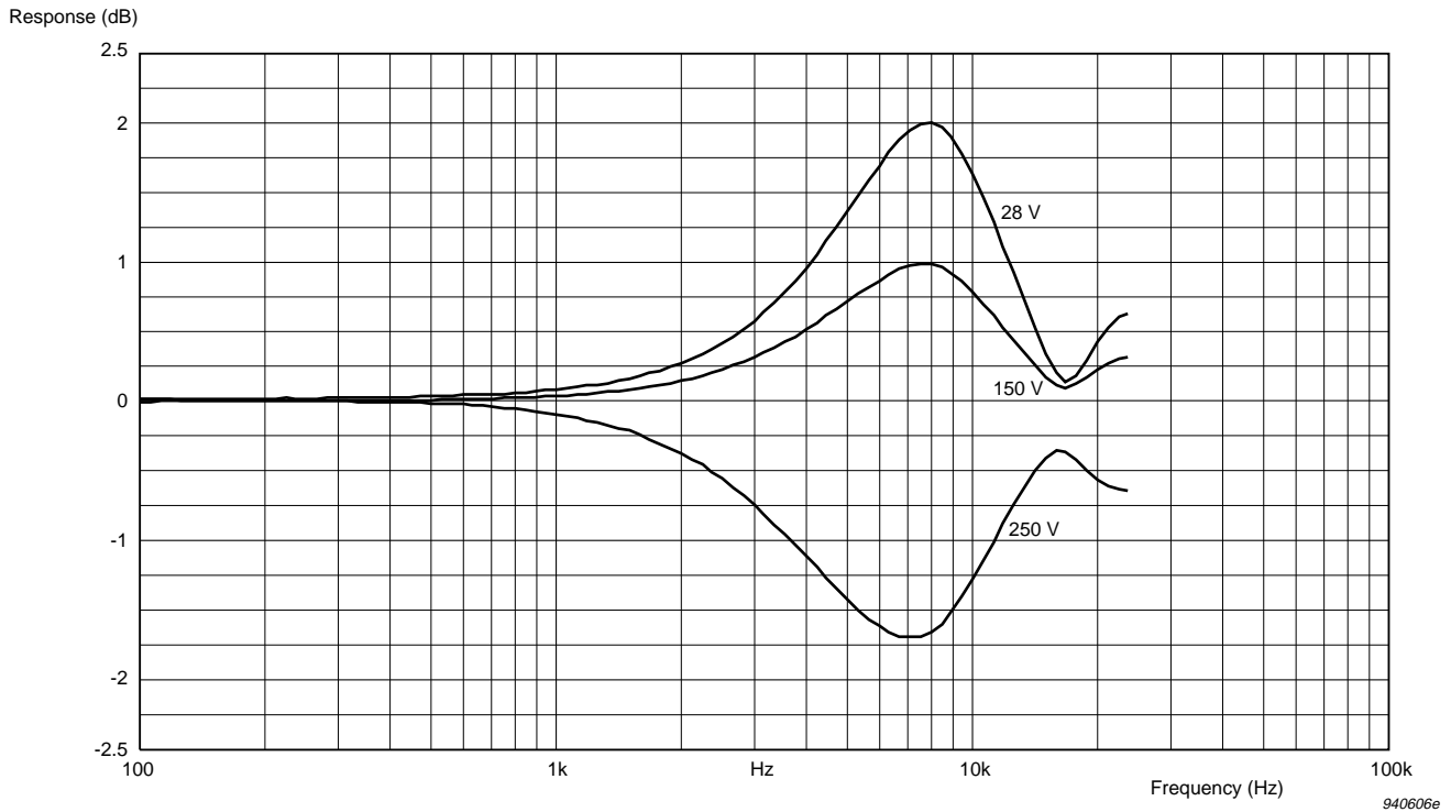
Fig. 3.7 Example of the frequency response dependency with polarisation voltage. The curves are normalised to the nominal value of 200 V. This example is for a 1/2 " microphone with high sensitivity. The dependency is less for 1/2 " microphones with lower sensitivity
