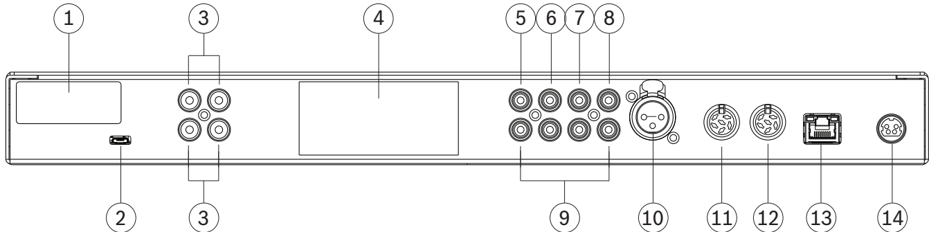
Figure 6.2: CCSD-CURDrear view
