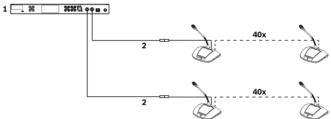
Figure 4.4: Example setup for a small/medium sized system (max. 80 discussion devices)
