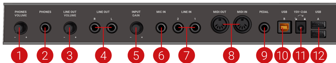
The rear panel
