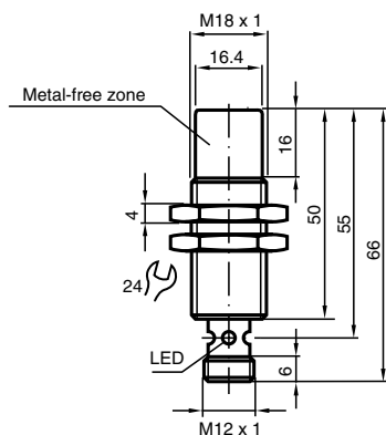
IQT-18GM-R4-V1-Y911215 dimension drawing
