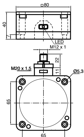
IQT-FP-R4-V1-Y911204 dimension drawing
