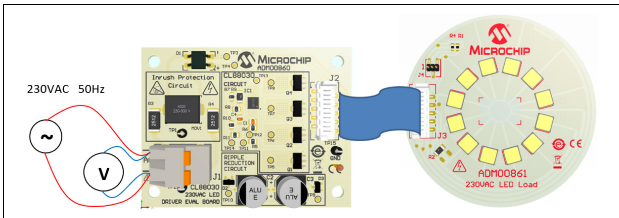
FIGURE 2-1: Connection Diagram.
