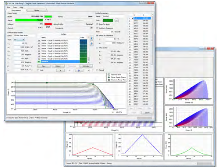
Magna-Power Electronics Photovoltaic Power Profile Emulation (PPPE) software: main program window (foreground); Viewer window (background)
