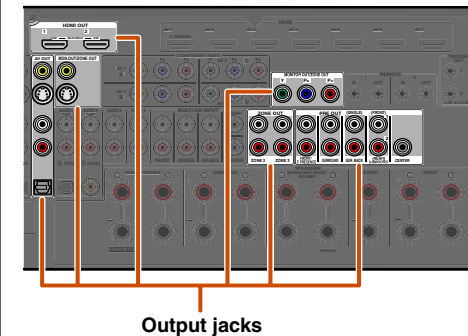
Output jacks
