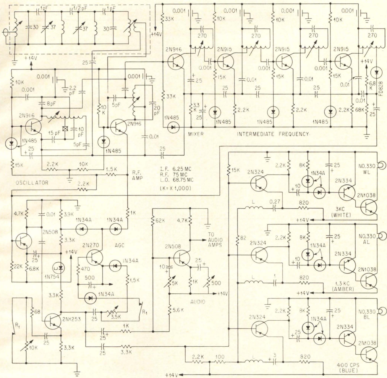
COMPACT design and layout features audio stage able to drive a multiple amplifier system. Indicator lights peak when over a marker beacon transmitter to aid in pinpointing position on airways or on an instrument-landing approach—Fig. 2
