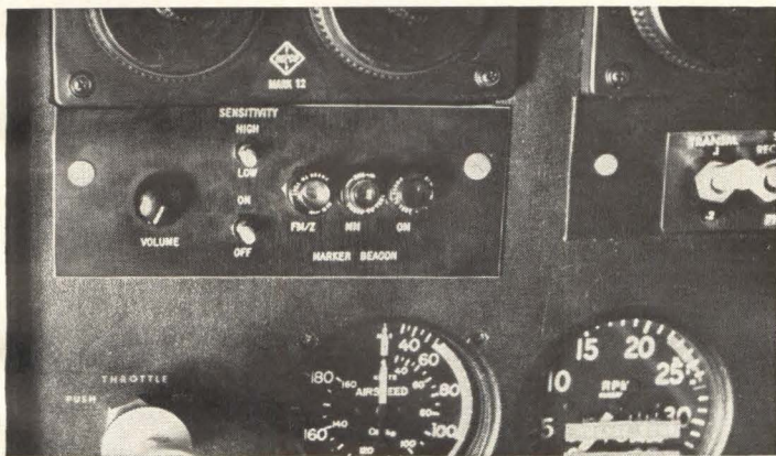
MARKER-BEACON RECEIVER controls mount on instrument panel 6¼ by 1½ by 1½ in. deep. Receiver is mounted in tail
