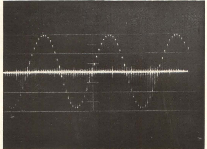
WAVEFORM of pulse-modulator output for 5-kc output
