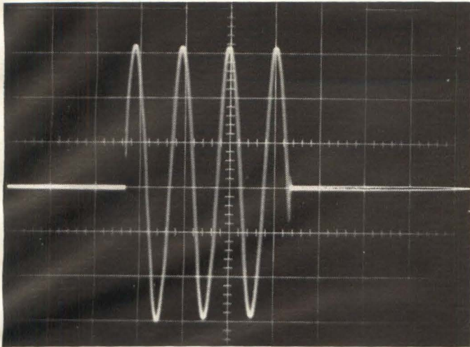
WAVEFORM of pulse-modulator output for 5-kc output
