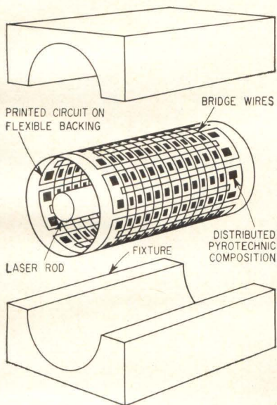
CONFIGURATION PROPOSED by Picatinny Arsenal scientists surrounds laser rod with pyrotechnic material. Printed circuit matrix ignites pyrotechnic material to produce simultaneous burning—Fig. 3
