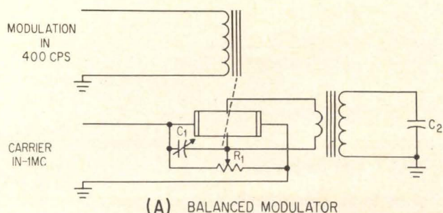
(A) BALANCED MODULATOR
