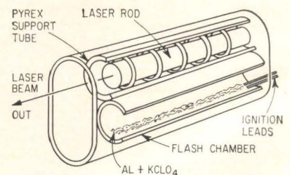
CONFIGURATION first lased by North American scientists in December 1962; a \frac{1}{4} -inch by 2-inch neodymium glass rod was used—Fig. 2
