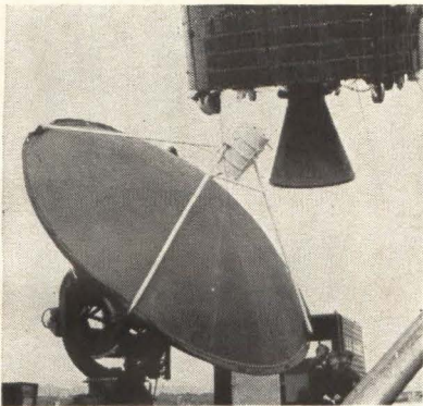
ANTENNA is air-inflated
