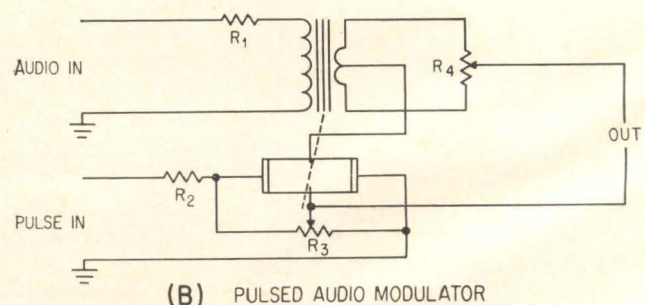
(B) PULSED AUDIO MODULATOR
