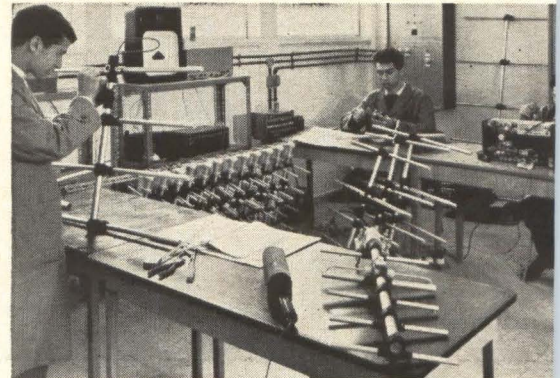
YAGI antennas under construction at Moshe Bassin
