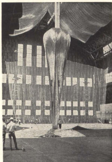
INFLATION TEST of Echo II. Balloon is 135 feet in diameter B
