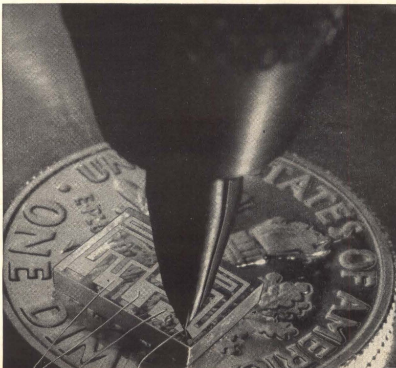
WELDER ELECTRONICS provides variable pulse trains by scr's to perform preheat and postheat of weldments. Voltage across electrodes is constantly monitored
