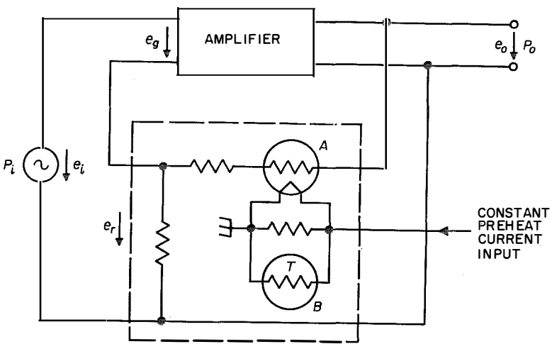
Figure 16—Basic circuit of controlled-gain group amplifier. Thermistor A determines the control characteristic and B the temperature balance. Amplification G = (e_o/e_i) \sim (e_o/e_r) .
