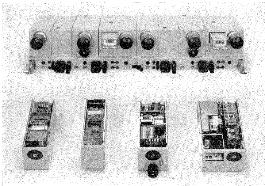
Figure 5—Channel converter panel with subassemblies.
