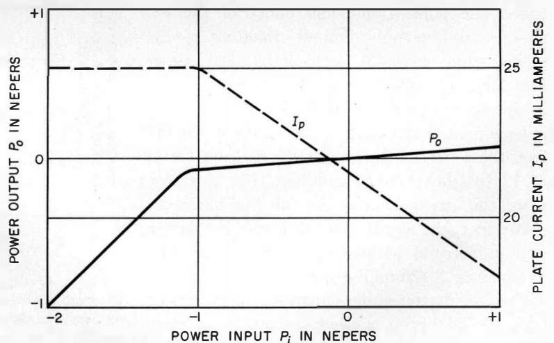
Figure 15—Characteristics of variable-gain channel amplifier.
