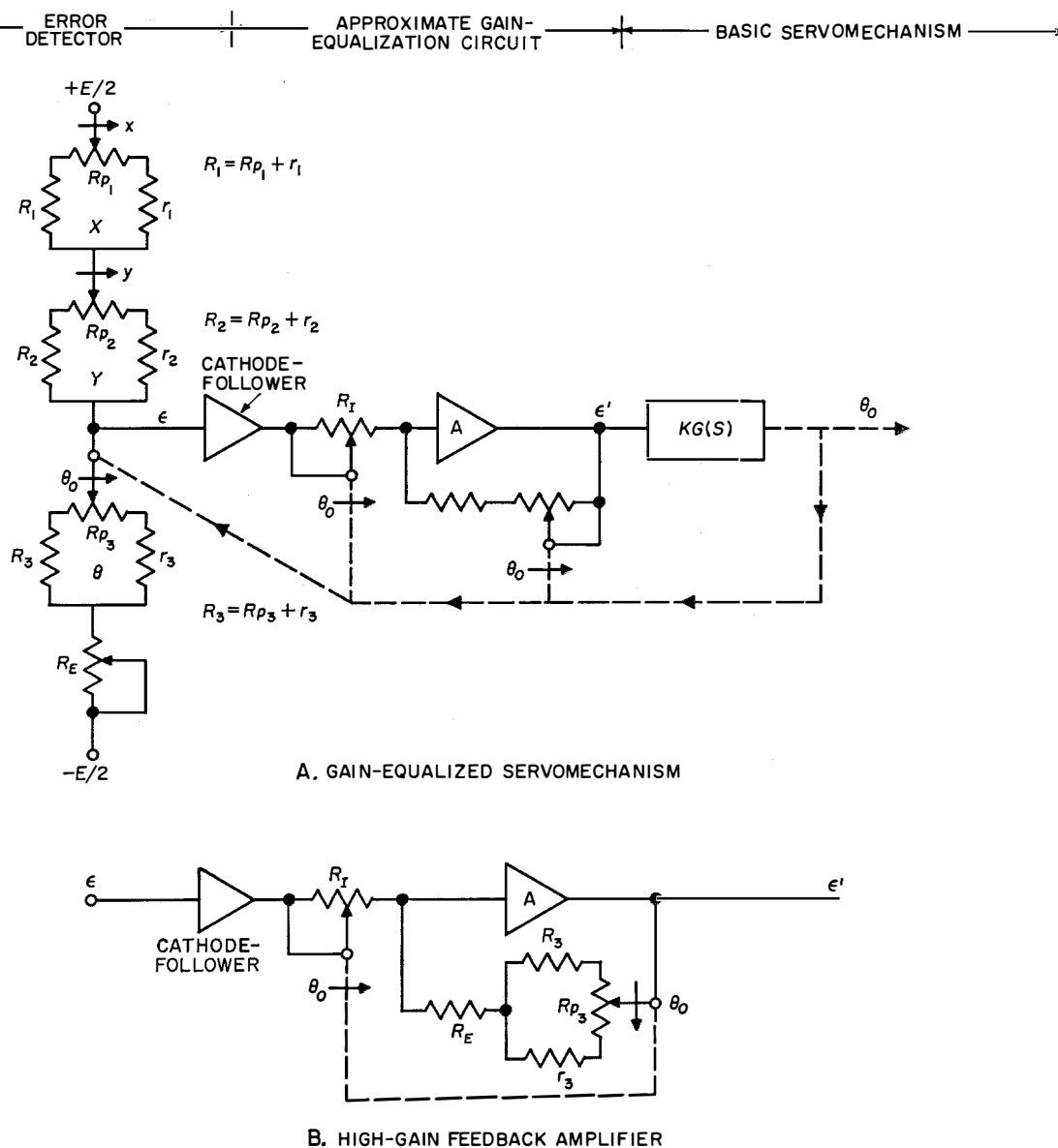
Figure 4—Diagram of square-root computer. In B,
