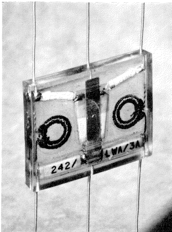
Type-242/LWA/3A suppressor.
