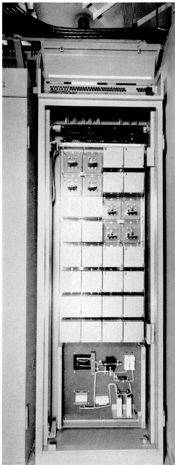
Figure 5—Cabinet mounting signaling relays and power supply, all of which are insulated to withstand 10-kilovolt faults.
