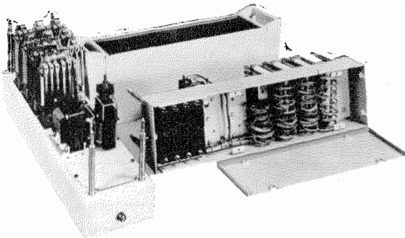
Figure 7—Typical relay arrangement.
