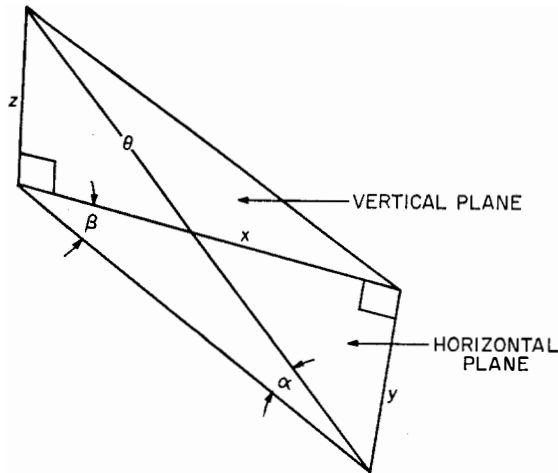
Figure 7—Vector diagram.
