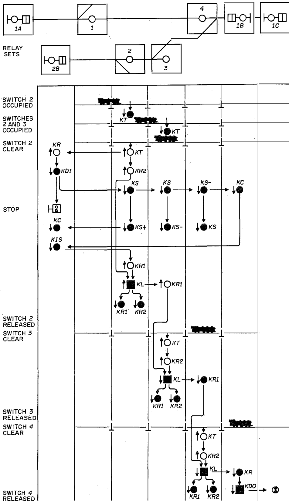
Figure 6—Release of switching elements after train has traversed the shunting route of Figure 5.
