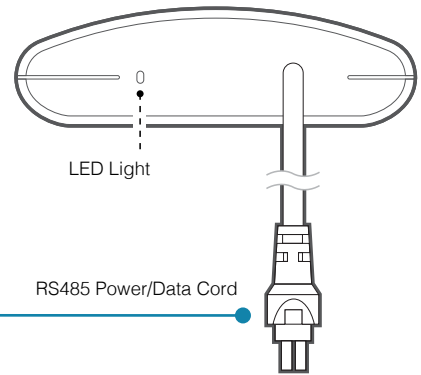
GATEWAY ULTRA Module (side view)
