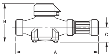
1-1/2" and 2" STANDARD MVR with Internal NPT ends
