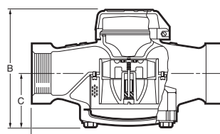
1-1/2" and 2" COMPACT MVR with Internal NPT ends
